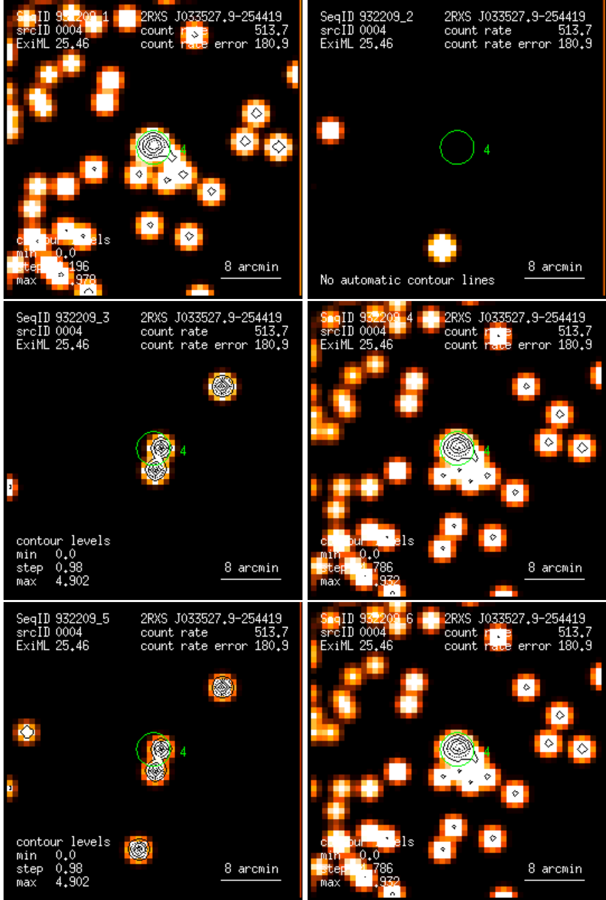
Figure 4: RASS 932209: detection 0004: band rate images, Gaussian filter: (1) PSPC channels 11 – 41, (2) 52 – 90, (3) 91 – 201, (4) 11 – 235, (5) 52 – 201, (6) 11 – 201. Broad band rates in counts/ks. Band rate contour levels in counts/ks/arcmin 2 .
