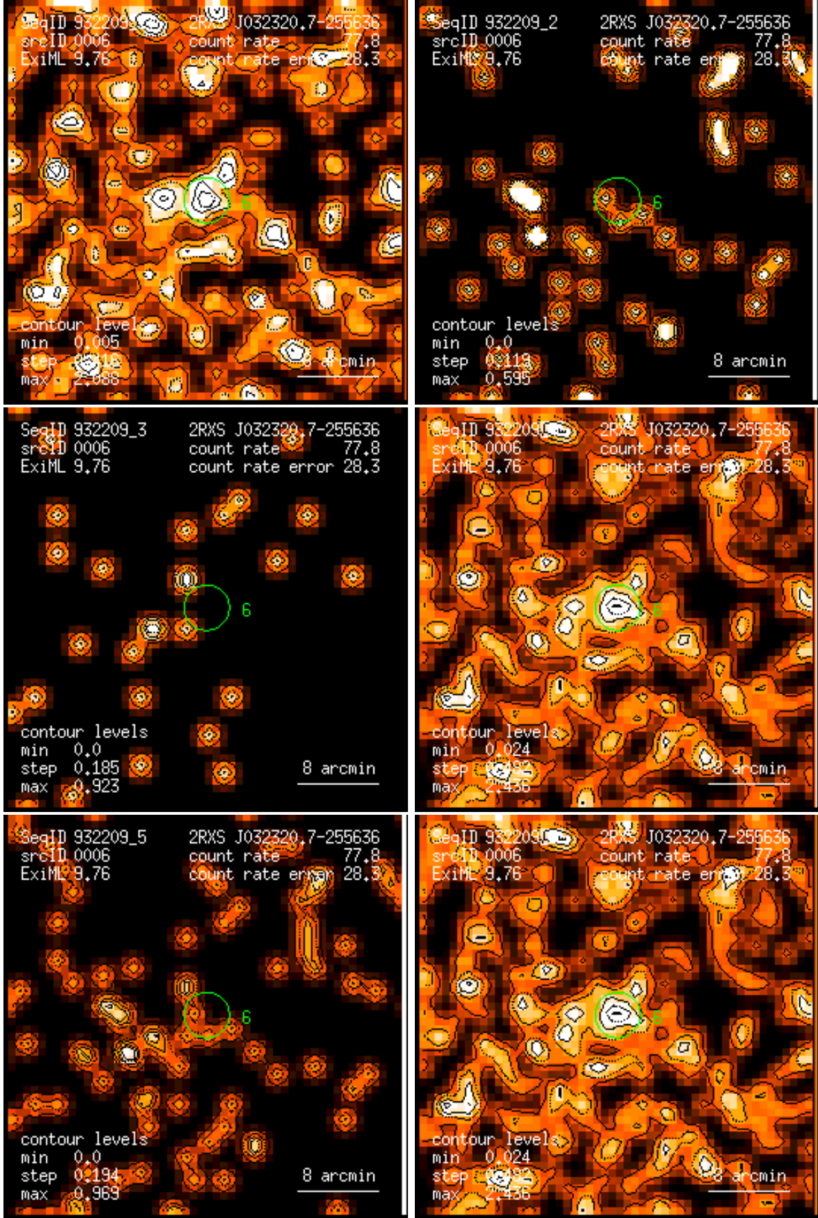
Figure 6: RASS 932209: detection 0006: band rate images, Gaussian filter: (1) PSPC channels 11 – 41, (2) 52 – 90, (3) 91 – 201, (4) 11 – 235, (5) 52 – 201, (6) 11 – 201. Broad band rates in counts/ks. Band rate contour levels in counts/ks/arcmin 2 .
