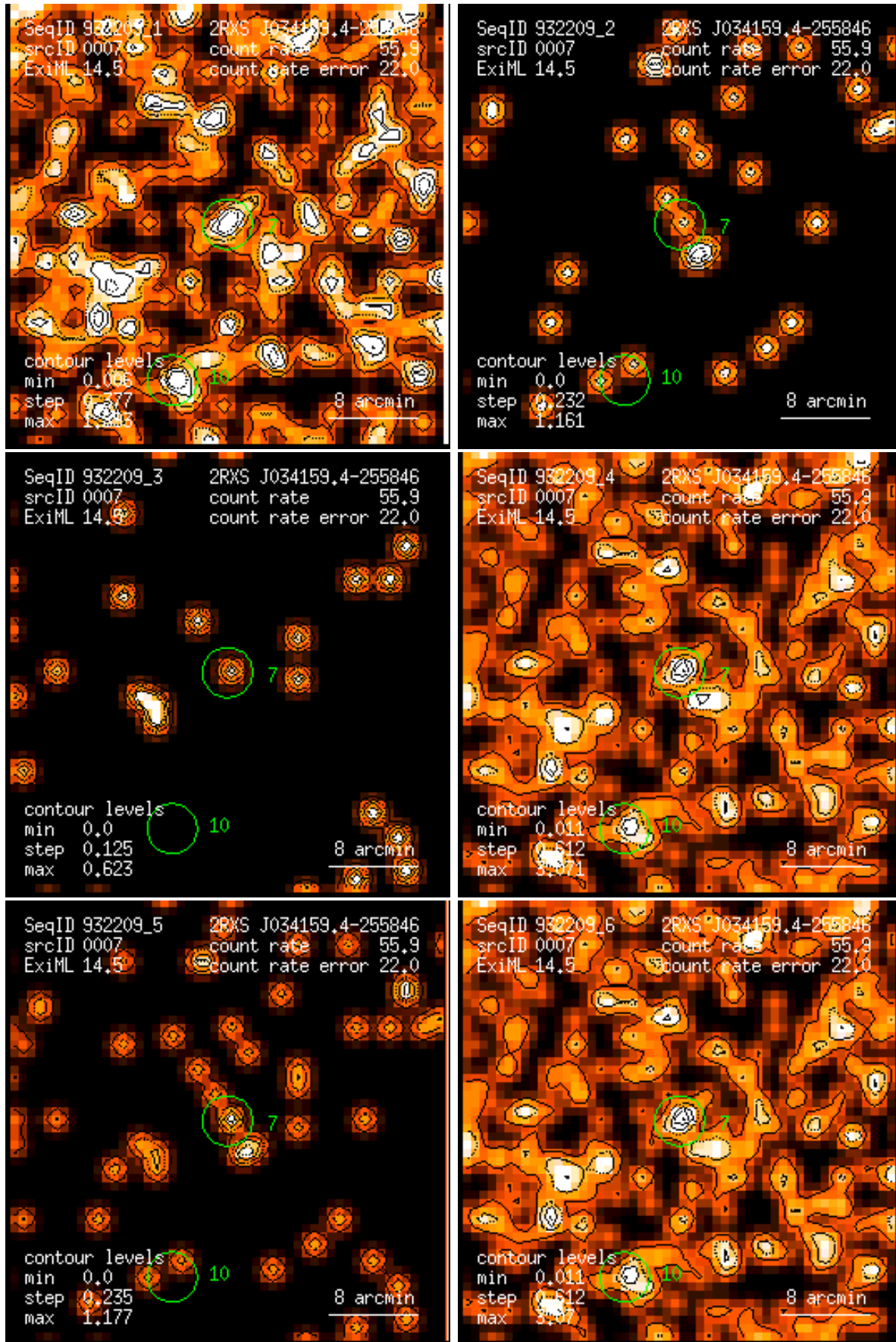
Figure 7: RASS 932209: detection 0007: band rate images, Gaussian filter: (1) PSPC channels 11 – 41, (2) 52 – 90, (3) 91 – 201, (4) 11 – 235, (5) 52 – 201, (6) 11 – 201. Broad band rates in counts/ks. Band rate contour levels in counts/ks/arcmin 2 .
