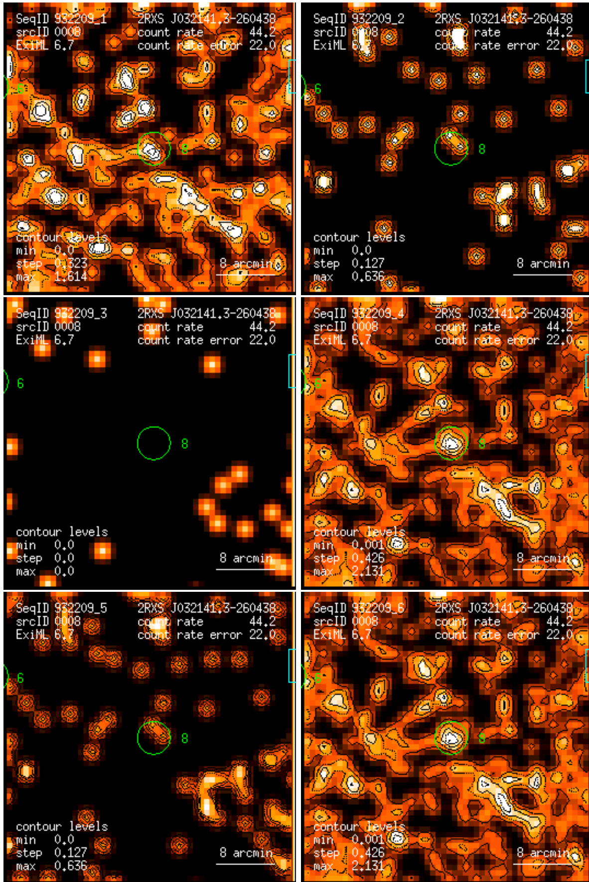
Figure 8: RASS 932209: detection 0008: band rate images, Gaussian filter: (1) PSPC channels 11 – 41, (2) 52 – 90, (3) 91 – 201, (4) 11 – 235, (5) 52 – 201, (6) 11 – 201. Broad band rates in counts/ks. Band rate contour levels in counts/ks/arcmin 2 .
