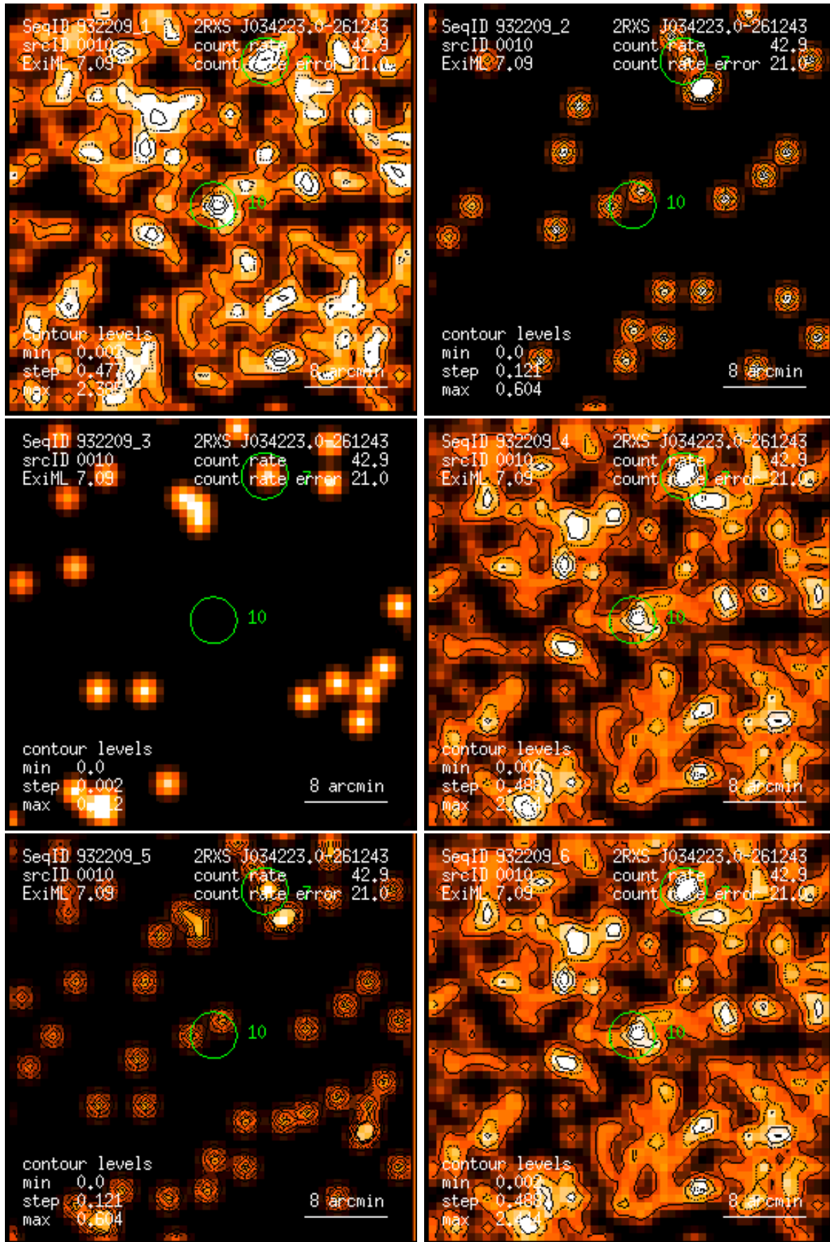
Figure 10: RASS 932209: detection 0010: band rate images, Gaussian filter: (1) PSPC channels 11 – 41, (2) 52 – 90, (3) 91 – 201, (4) 11 – 235, (5) 52 – 201, (6) 11 – 201. Broad band rates in counts/ks. Band rate contour levels in counts/ks/arcmin 2 .
