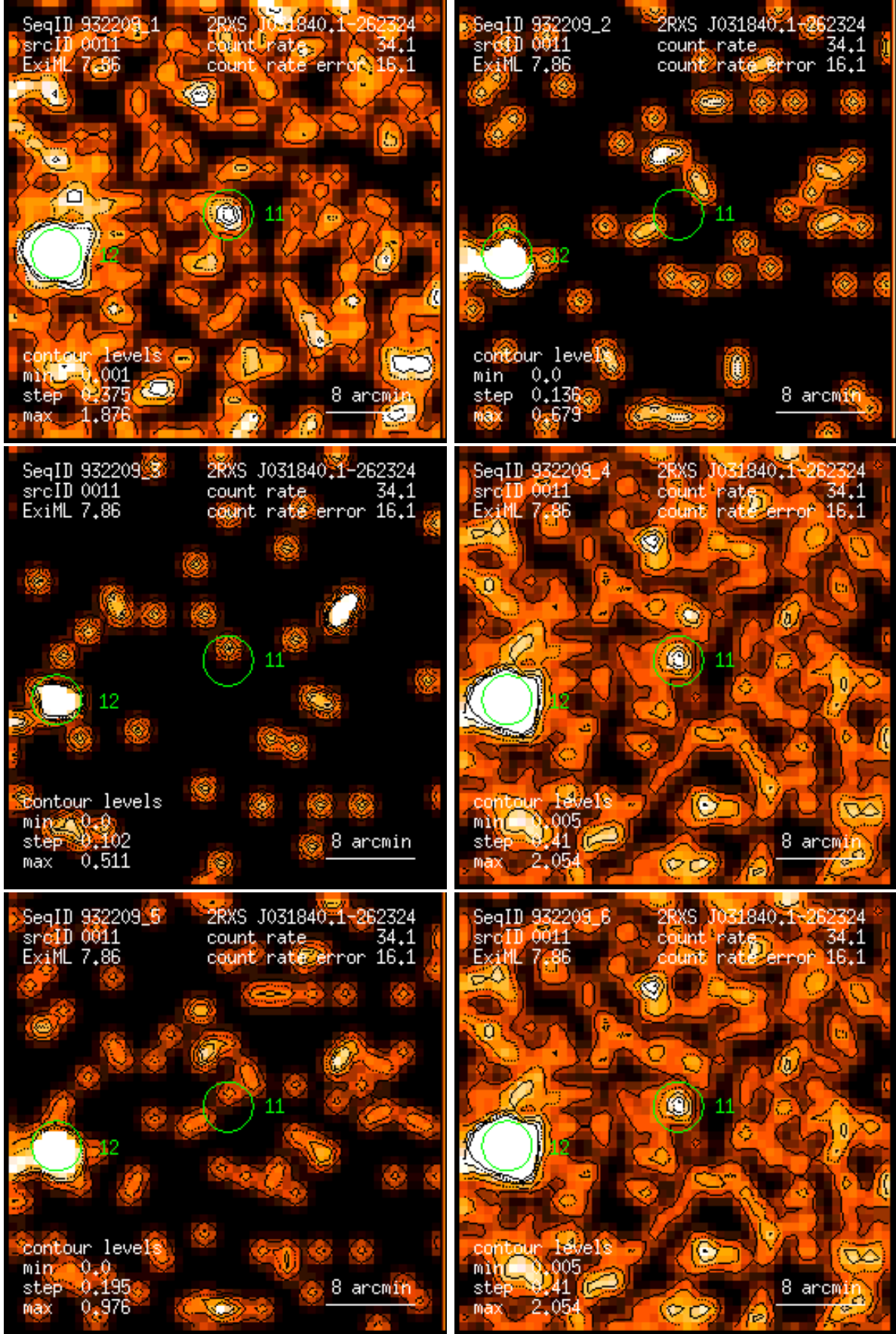
Figure 11: RASS 932209: detection 0011: band rate images, Gaussian filter: (1) PSPC channels 11 – 41, (2) 52 – 90, (3) 91 – 201, (4) 11 – 235, (5) 52 – 201, (6) 11 – 201. Broad band rates in counts/ks. Band rate contour levels in counts/ks/arcmin 2 .
