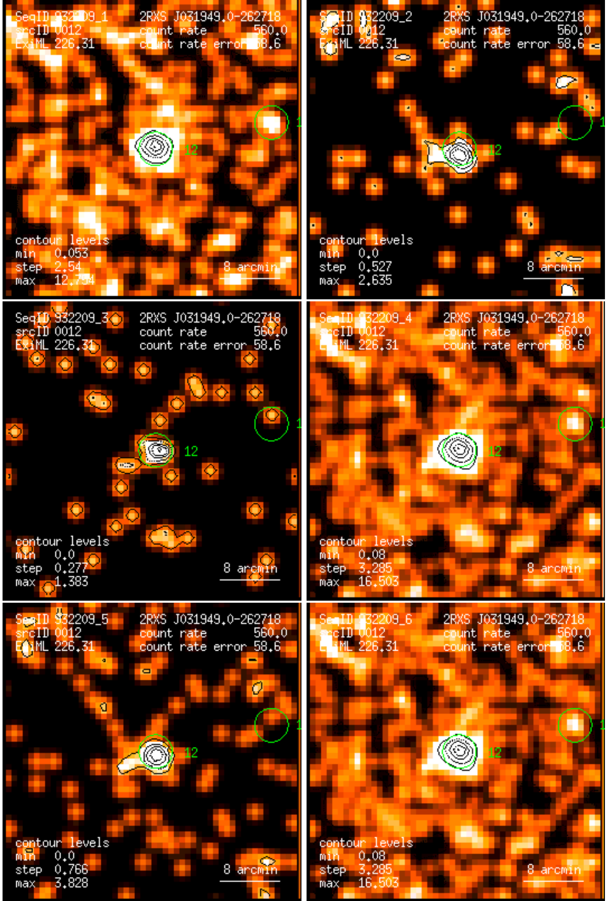
Figure 12: RASS 932209: detection 0012: band rate images, Gaussian filter: (1) PSPC channels 11 – 41, (2) 52 – 90, (3) 91 – 201, (4) 11 – 235, (5) 52 – 201, (6) 11 – 201. Broad band rates in counts/ks. Band rate contour levels in counts/ks/arcmin 2 .
