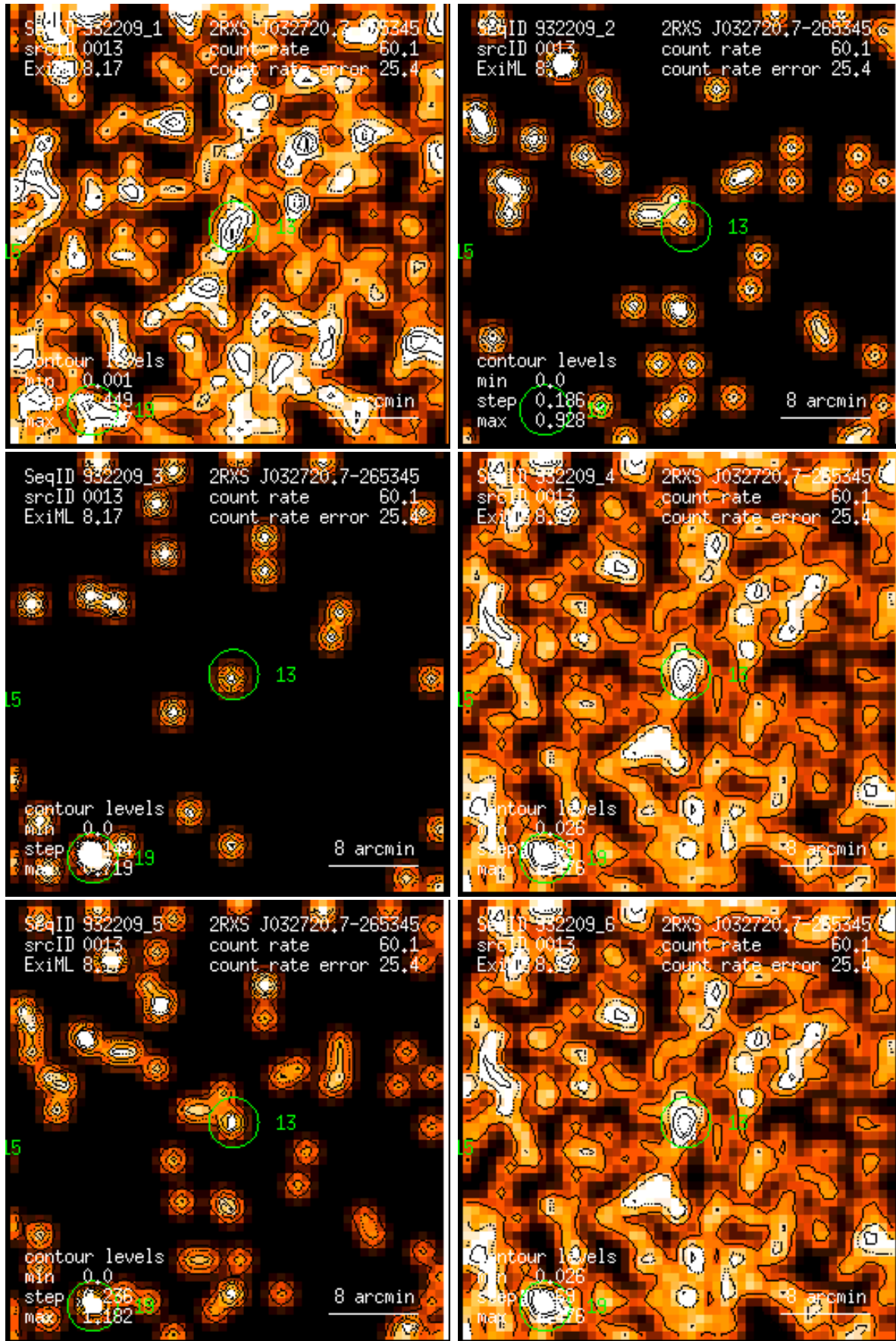
Figure 13: RASS 932209: detection 0013: band rate images, Gaussian filter: (1) PSPC channels 11 – 41, (2) 52 – 90, (3) 91 – 201, (4) 11 – 235, (5) 52 – 201, (6) 11 – 201. Broad band rates in counts/ks. Band rate contour levels in counts/ks/arcmin 2 .
