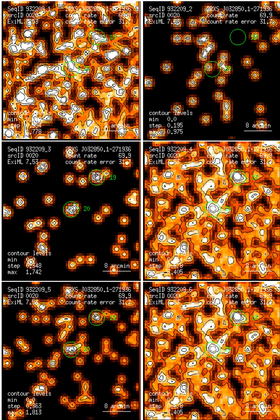
Figure 20: RASS 932209: detection 0020: band rate images, Gaussian filter: (1) PSPC channels 11 – 41, (2) 52 – 90, (3) 91 – 201, (4) 11 – 235, (5) 52 – 201, (6) 11 – 201. Broad band rates in counts/ks. Band rate contour levels in counts/ks/arcmin 2 .
