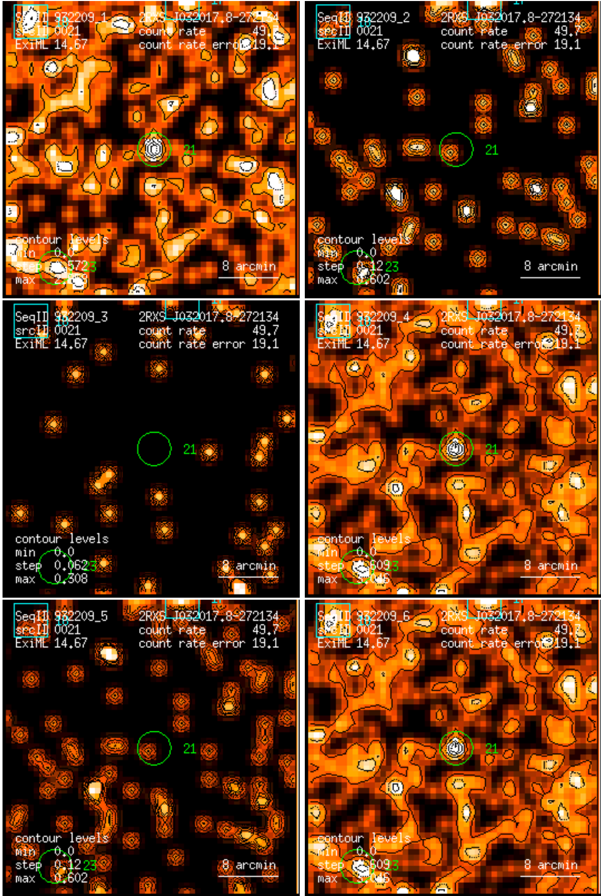
Figure 21: RASS 932209: detection 0021: band rate images, Gaussian filter: (1) PSPC channels 11 – 41, (2) 52 – 90, (3) 91 – 201, (4) 11 – 235, (5) 52 – 201, (6) 11 – 201. Broad band rates in counts/ks. Band rate contour levels in counts/ks/arcmin 2 .
