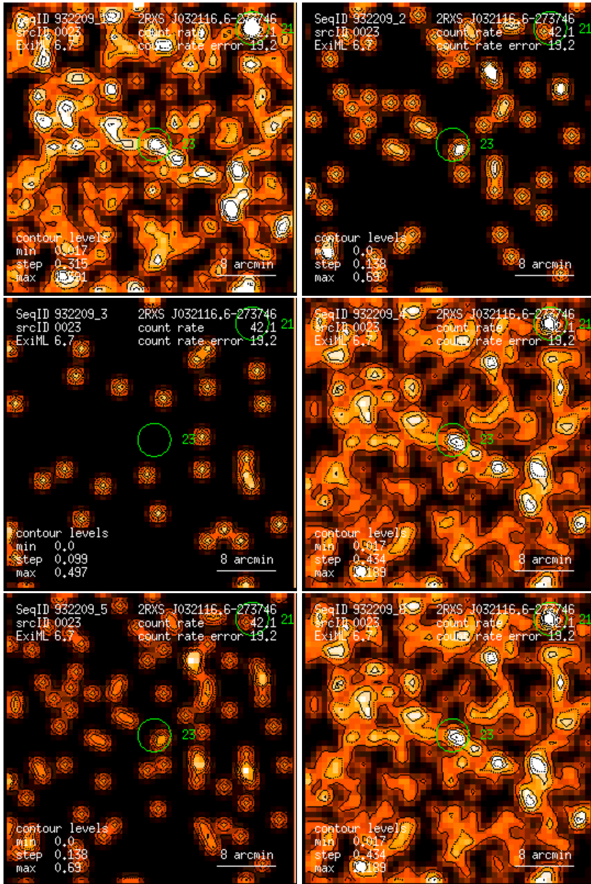
Figure 23: RASS 932209: detection 0023: band rate images, Gaussian filter: (1) PSPC channels 11 – 41, (2) 52 – 90, (3) 91 – 201, (4) 11 – 235, (5) 52 – 201, (6) 11 – 201. Broad band rates in counts/ks. Band rate contour levels in counts/ks/arcmin 2 .
