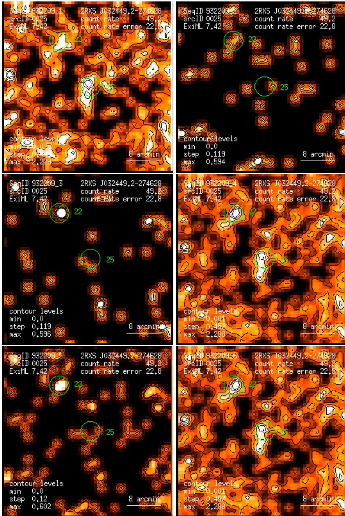
Figure 25: RASS 932209: detection 0025: band rate images, Gaussian filter: (1) PSPC channels 11 – 41, (2) 52 – 90, (3) 91 – 201, (4) 11 – 235, (5) 52 – 201, (6) 11 – 201. Broad band rates in counts/ks. Band rate contour levels in counts/ks/arcmin 2 .
