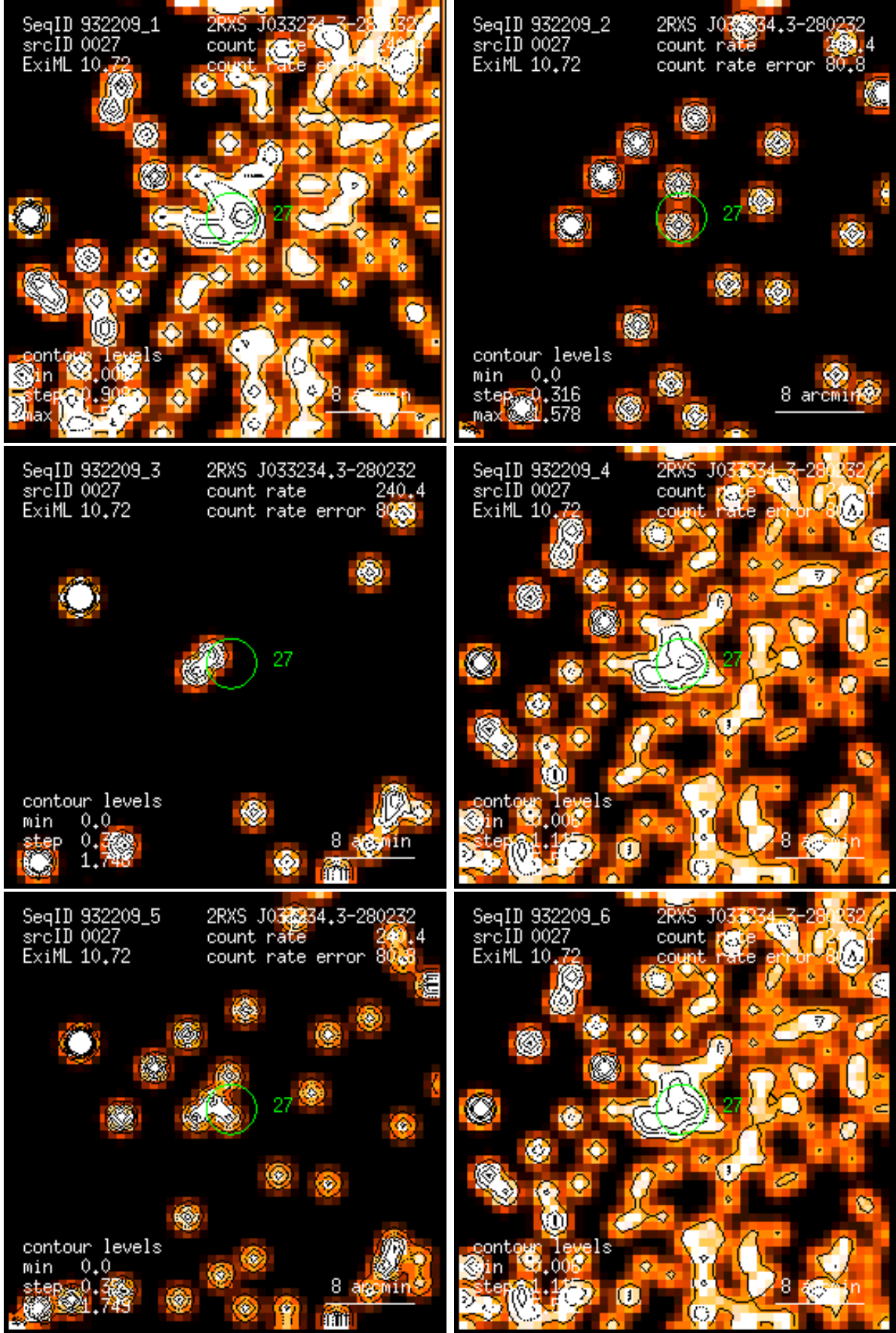
Figure 27: RASS 932209: detection 0027: band rate images, Gaussian filter: (1) PSPC channels 11 – 41, (2) 52 – 90, (3) 91 – 201, (4) 11 – 235, (5) 52 – 201, (6) 11 – 201. Broad band rates in counts/ks. Band rate contour levels in counts/ks/arcmin 2 .
