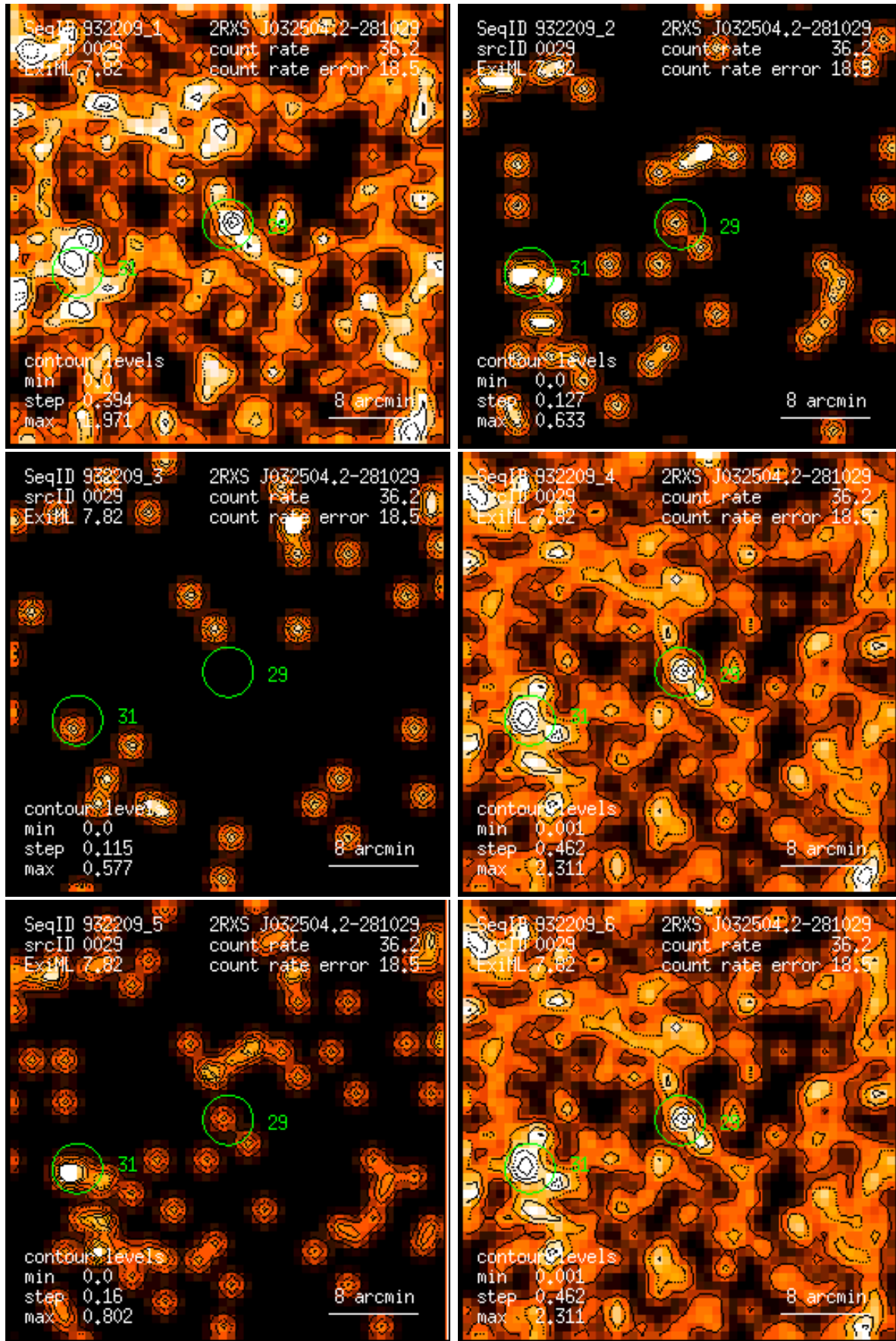
Figure 29: RASS 932209: detection 0029: band rate images, Gaussian filter: (1) PSPC channels 11 – 41, (2) 52 – 90, (3) 91 – 201, (4) 11 – 235, (5) 52 – 201, (6) 11 – 201. Broad band rates in counts/ks. Band rate contour levels in counts/ks/arcmin 2 .
