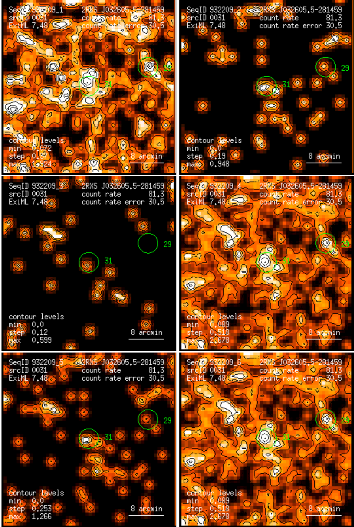
Figure 31: RASS 932209: detection 0031: band rate images, Gaussian filter: (1) PSPC channels 11 – 41, (2) 52 – 90, (3) 91 – 201, (4) 11 – 235, (5) 52 – 201, (6) 11 – 201. Broad band rates in counts/ks. Band rate contour levels in counts/ks/arcmin 2 .
