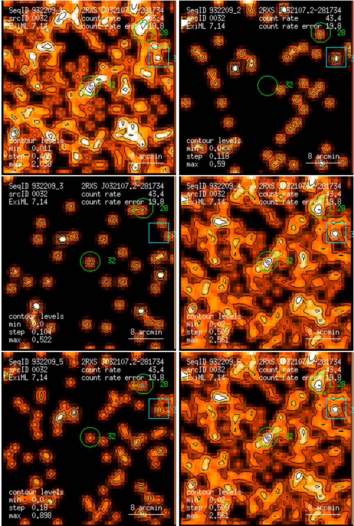
Figure 32: RASS 932209: detection 0032: band rate images, Gaussian filter: (1) PSPC channels 11 – 41, (2) 52 – 90, (3) 91 – 201, (4) 11 – 235, (5) 52 – 201, (6) 11 – 201. Broad band rates in counts/ks. Band rate contour levels in counts/ks/arcmin 2 .
