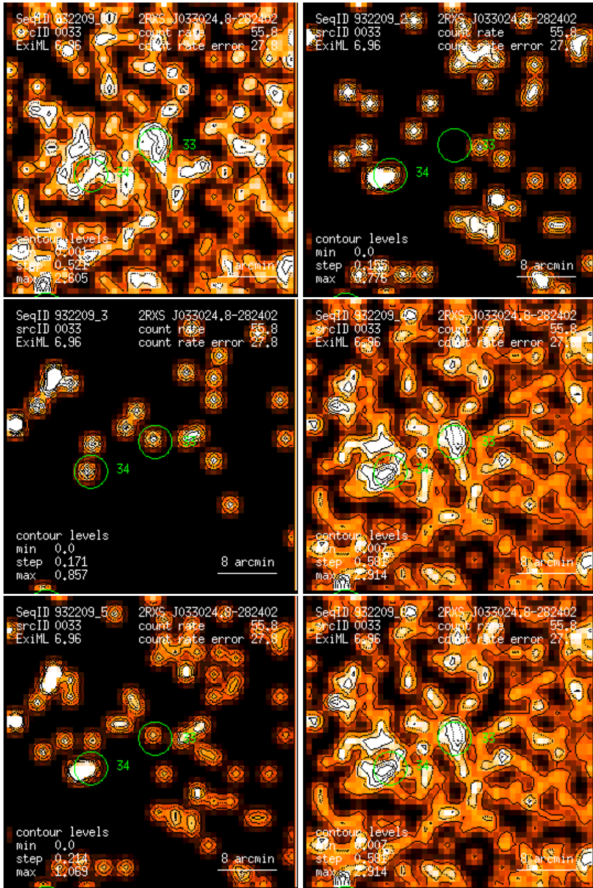
Figure 33: RASS 932209: detection 0033: band rate images, Gaussian filter: (1) PSPC channels 11 – 41, (2) 52 – 90, (3) 91 – 201, (4) 11 – 235, (5) 52 – 201, (6) 11 – 201. Broad band rates in counts/ks. Band rate contour levels in counts/ks/arcmin 2 .
