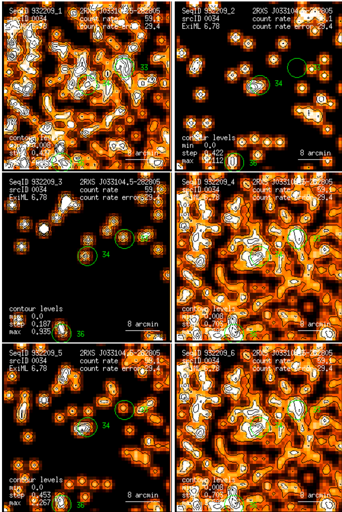
Figure 34: RASS 932209: detection 0034: band rate images, Gaussian filter: (1) PSPC channels 11 – 41, (2) 52 – 90, (3) 91 – 201, (4) 11 – 235, (5) 52 – 201, (6) 11 – 201. Broad band rates in counts/ks. Band rate contour levels in counts/ks/arcmin 2 .
