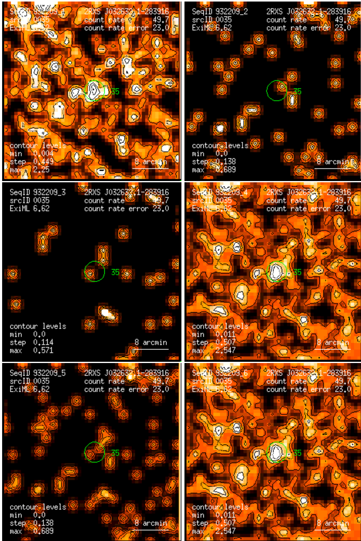
Figure 35: RASS 932209: detection 0035: band rate images, Gaussian filter: (1) PSPC channels 11 – 41, (2) 52 – 90, (3) 91 – 201, (4) 11 – 235, (5) 52 – 201, (6) 11 – 201. Broad band rates in counts/ks. Band rate contour levels in counts/ks/arcmin 2 .
