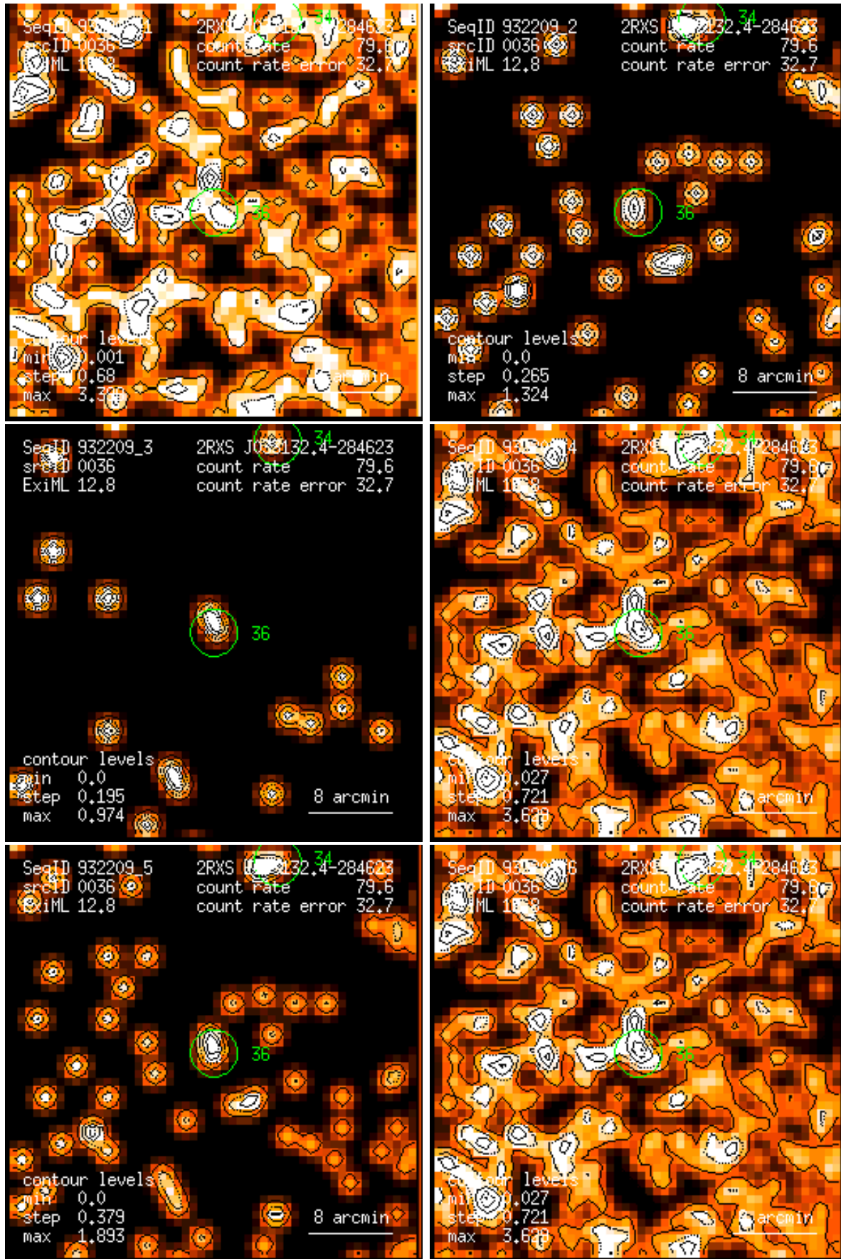
Figure 36: RASS 932209: detection 0036: band rate images, Gaussian filter: (1) PSPC channels 11 – 41, (2) 52 – 90, (3) 91 – 201, (4) 11 – 235, (5) 52 – 201, (6) 11 – 201. Broad band rates in counts/ks. Band rate contour levels in counts/ks/arcmin 2 .
