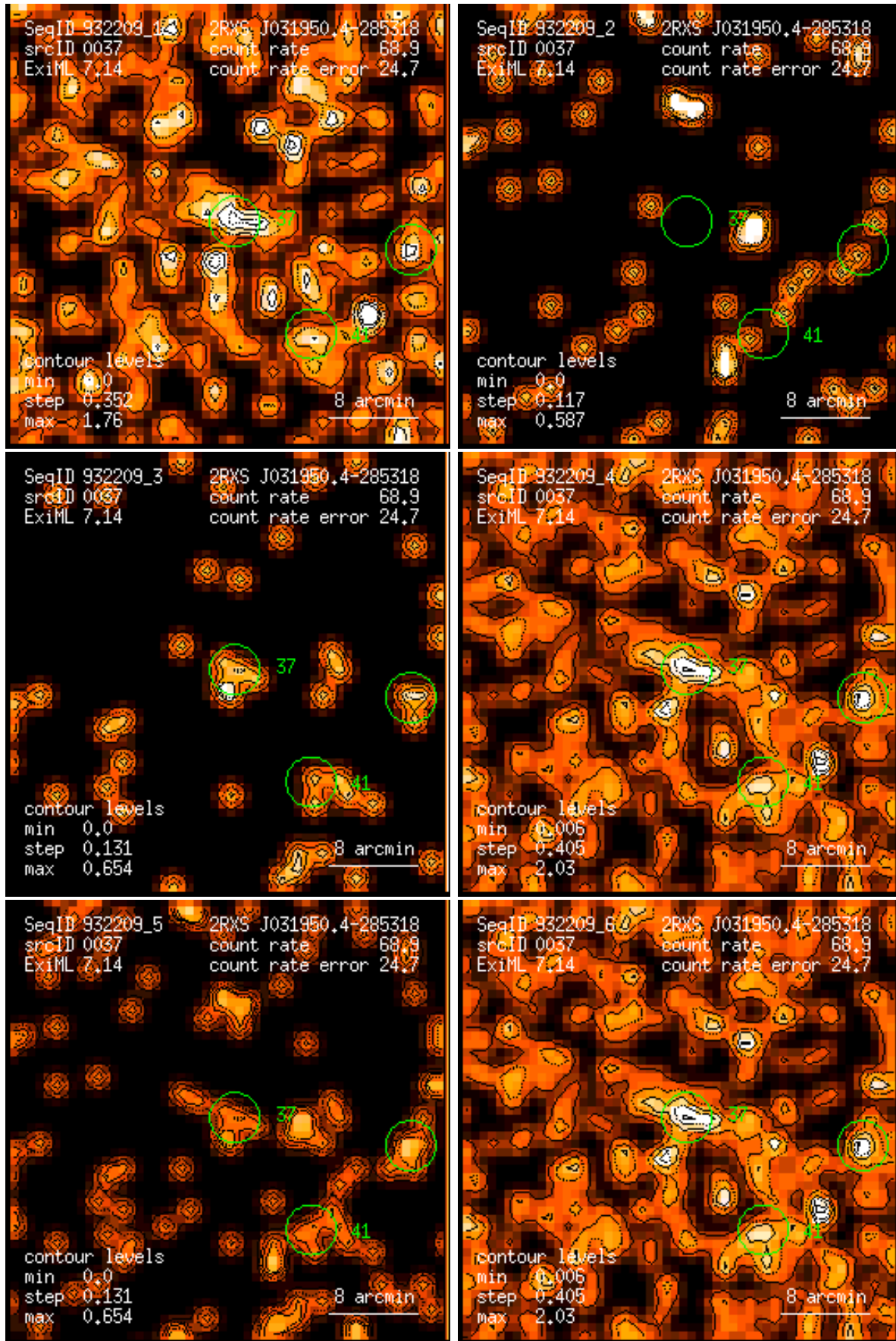
Figure 37: RASS 932209: detection 0037: band rate images, Gaussian filter: (1) PSPC channels 11 – 41, (2) 52 – 90, (3) 91 – 201, (4) 11 – 235, (5) 52 – 201, (6) 11 – 201. Broad band rates in counts/ks. Band rate contour levels in counts/ks/arcmin 2 .
