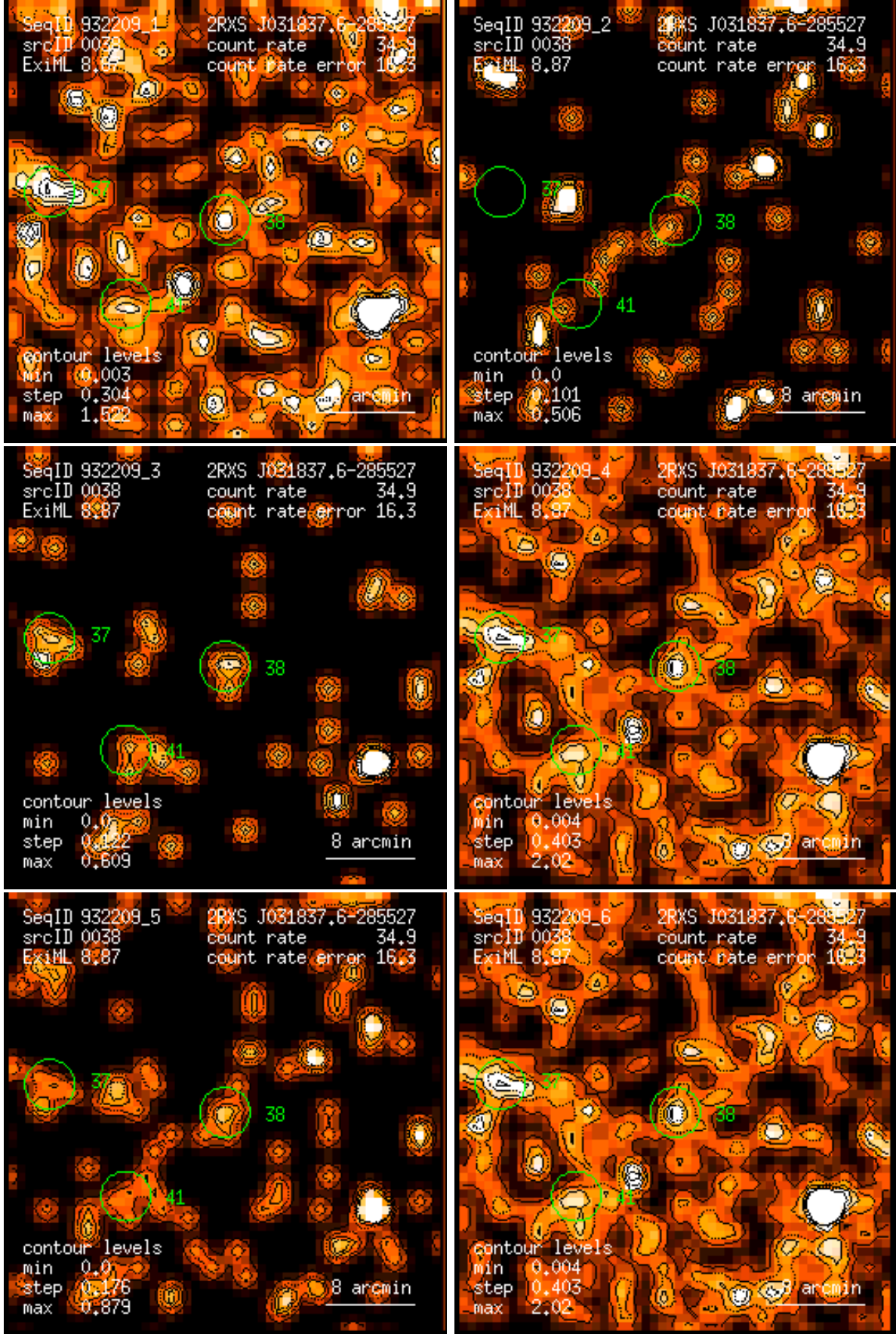
Figure 38: RASS 932209: detection 0038: band rate images, Gaussian filter: (1) PSPC channels 11 – 41, (2) 52 – 90, (3) 91 – 201, (4) 11 – 235, (5) 52 – 201, (6) 11 – 201. Broad band rates in counts/ks. Band rate contour levels in counts/ks/arcmin 2 .
