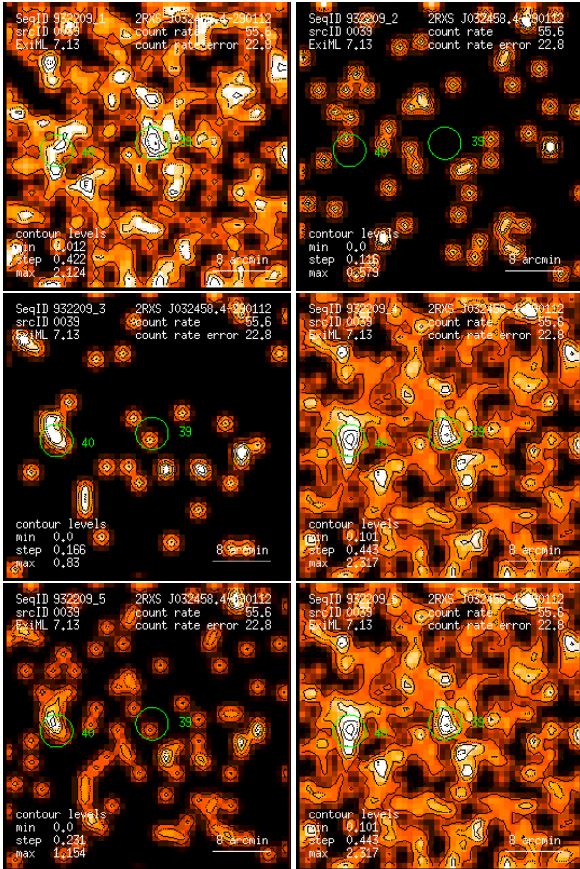
Figure 39: RASS 932209: detection 0039: band rate images, Gaussian filter: (1) PSPC channels 11 – 41, (2) 52 – 90, (3) 91 – 201, (4) 11 – 235, (5) 52 – 201, (6) 11 – 201. Broad band rates in counts/ks. Band rate contour levels in counts/ks/arcmin 2 .
