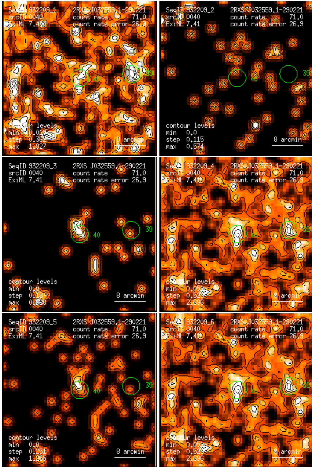
Figure 40: RASS 932209: detection 0040: band rate images, Gaussian filter: (1) PSPC channels 11 – 41, (2) 52 – 90, (3) 91 – 201, (4) 11 – 235, (5) 52 – 201, (6) 11 – 201. Broad band rates in counts/ks. Band rate contour levels in counts/ks/arcmin 2 .
