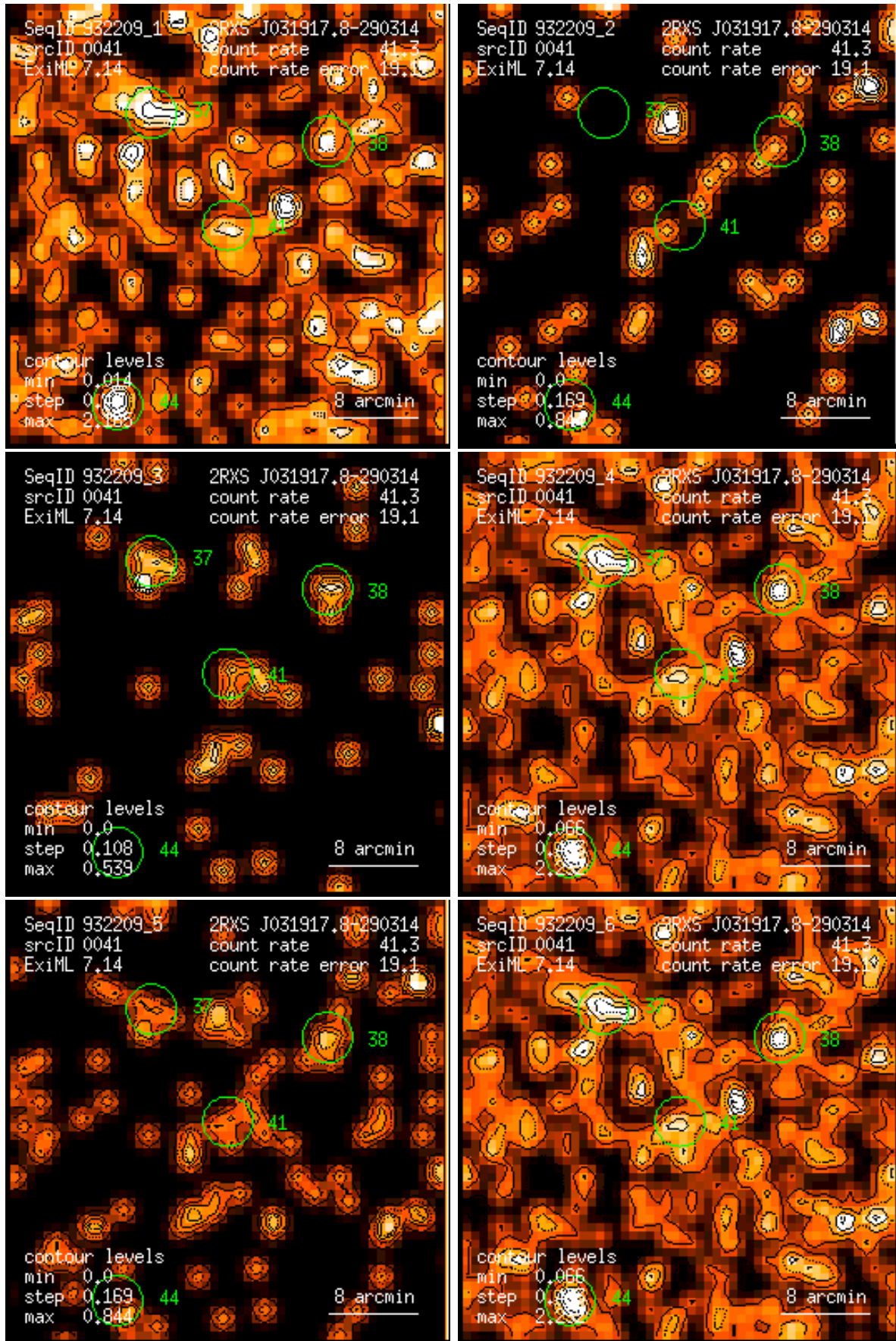
Figure 41: RASS 932209: detection 0041: band rate images, Gaussian filter: (1) PSPC channels 11 – 41, (2) 52 – 90, (3) 91 – 201, (4) 11 – 235, (5) 52 – 201, (6) 11 – 201. Broad band rates in counts/ks. Band rate contour levels in counts/ks/arcmin 2 .
