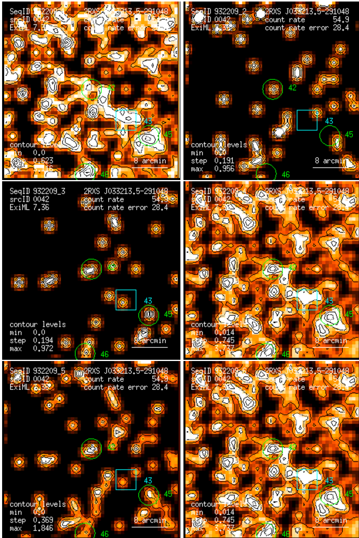
Figure 42: RASS 932209: detection 0042: band rate images, Gaussian filter: (1) PSPC channels 11 – 41, (2) 52 – 90, (3) 91 – 201, (4) 11 – 235, (5) 52 – 201, (6) 11 – 201. Broad band rates in counts/ks. Band rate contour levels in counts/ks/arcmin 2 .
