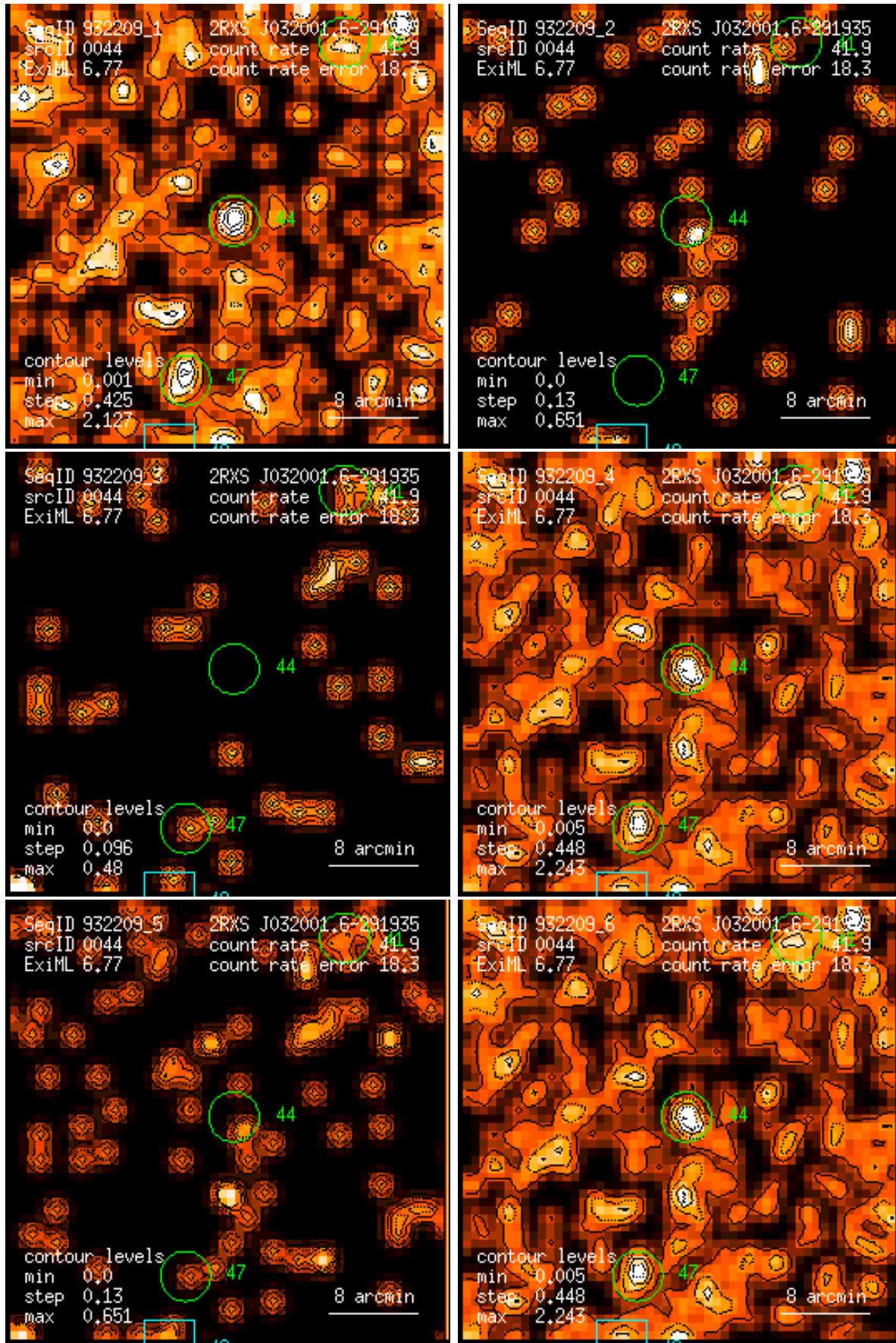
Figure 44: RASS 932209: detection 0044: band rate images, Gaussian filter: (1) PSPC channels 11 – 41, (2) 52 – 90, (3) 91 – 201, (4) 11 – 235, (5) 52 – 201, (6) 11 – 201. Broad band rates in counts/ks. Band rate contour levels in counts/ks/arcmin 2 .
