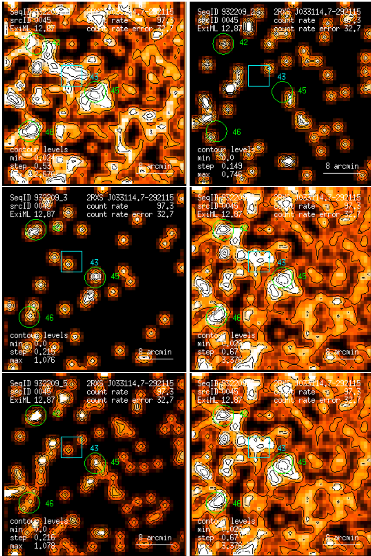
Figure 45: RASS 932209: detection 0045: band rate images, Gaussian filter: (1) PSPC channels 11 – 41, (2) 52 – 90, (3) 91 – 201, (4) 11 – 235, (5) 52 – 201, (6) 11 – 201. Broad band rates in counts/ks. Band rate contour levels in counts/ks/arcmin 2 .
