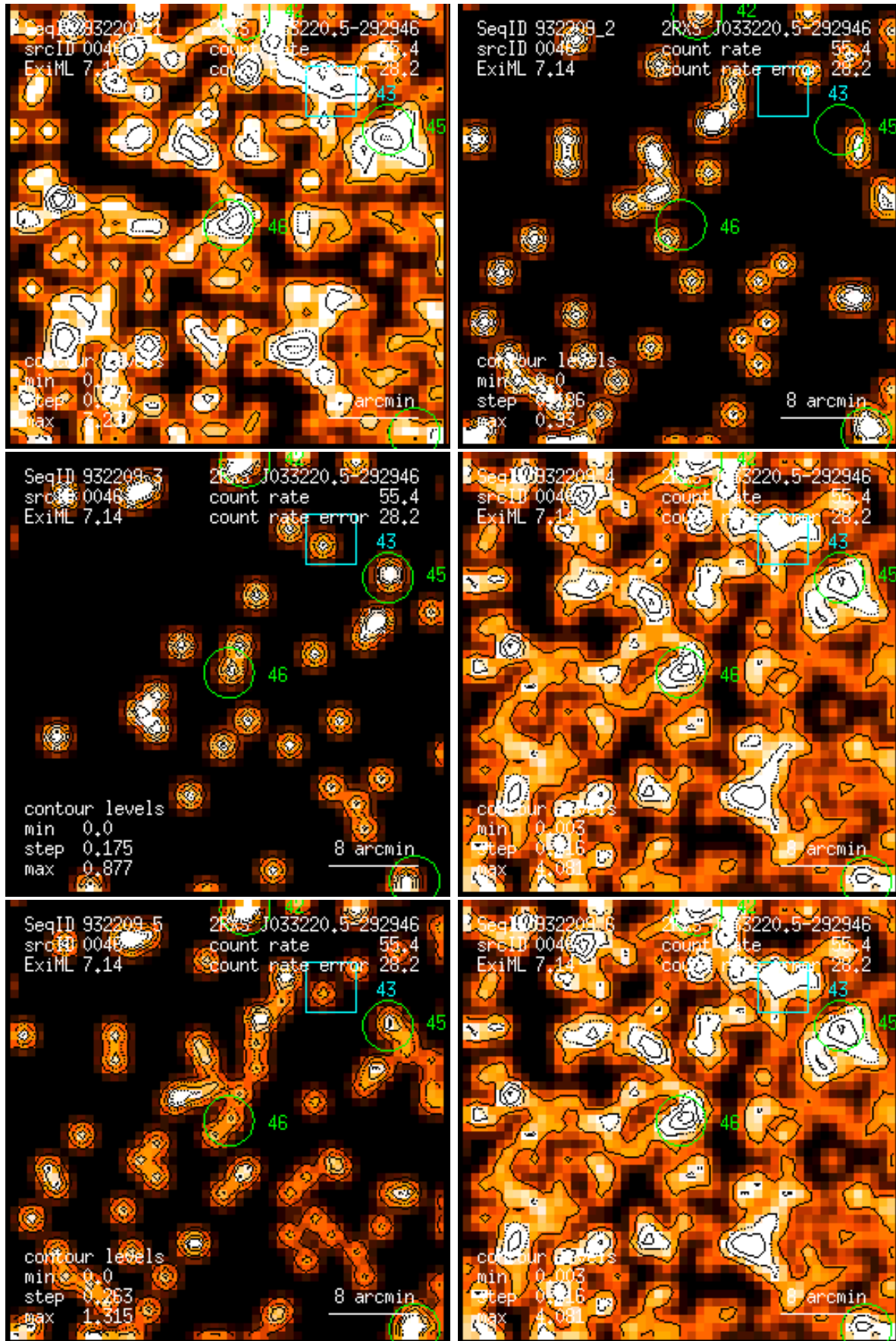
Figure 46: RASS 932209: detection 0046: band rate images, Gaussian filter: (1) PSPC channels 11 – 41, (2) 52 – 90, (3) 91 – 201, (4) 11 – 235, (5) 52 – 201, (6) 11 – 201. Broad band rates in counts/ks. Band rate contour levels in counts/ks/arcmin 2 .
