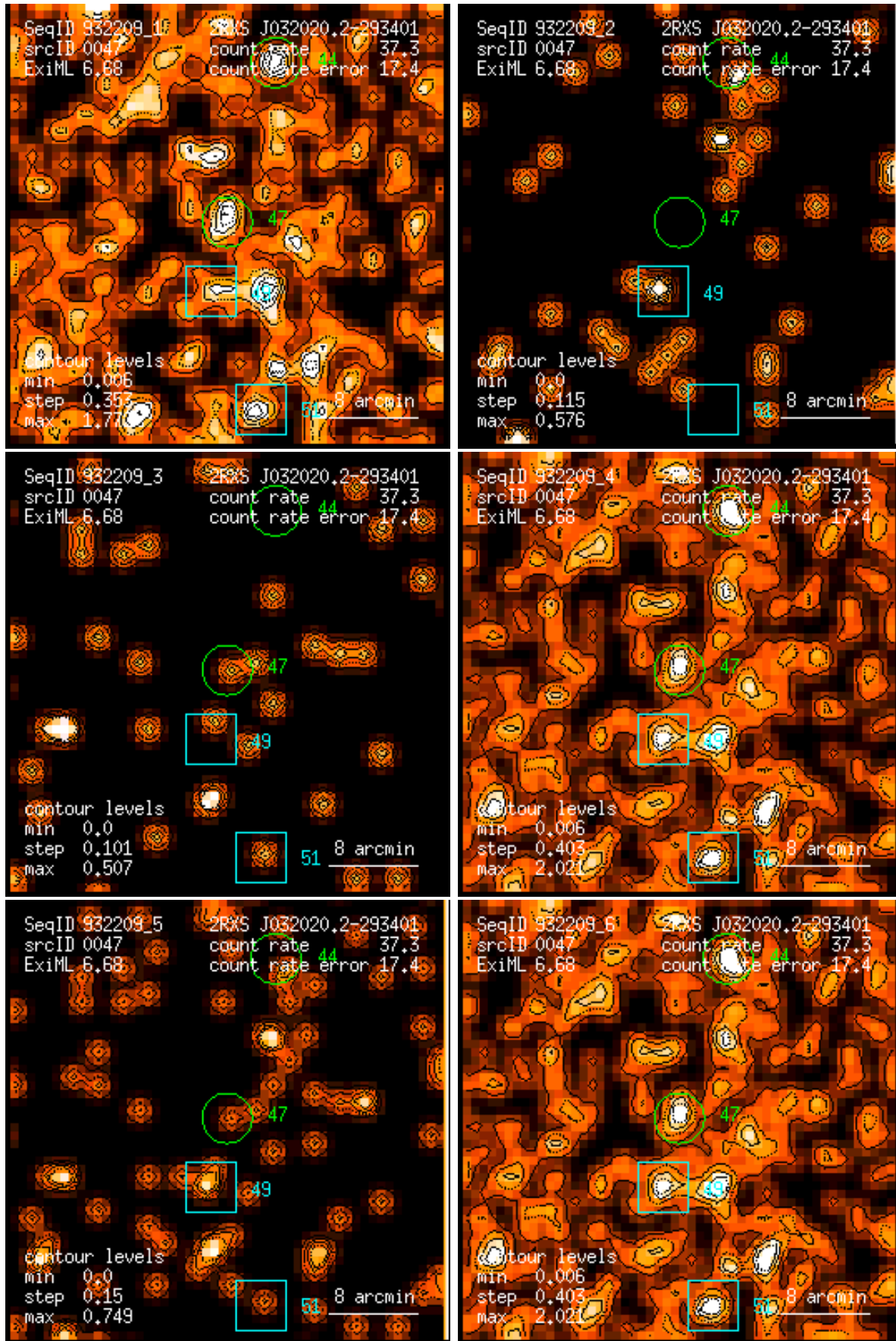
Figure 47: RASS 932209: detection 0047: band rate images, Gaussian filter: (1) PSPC channels 11 – 41, (2) 52 – 90, (3) 91 – 201, (4) 11 – 235, (5) 52 – 201, (6) 11 – 201. Broad band rates in counts/ks. Band rate contour levels in counts/ks/arcmin 2 .
