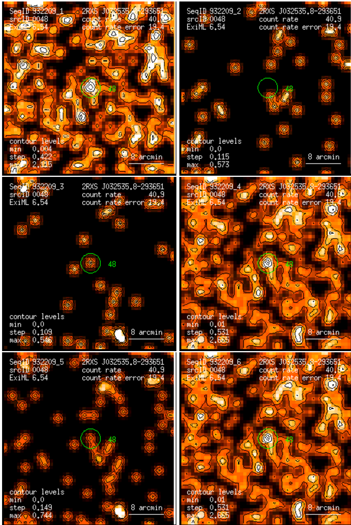
Figure 48: RASS 932209: detection 0048: band rate images, Gaussian filter: (1) PSPC channels 11 – 41, (2) 52 – 90, (3) 91 – 201, (4) 11 – 235, (5) 52 – 201, (6) 11 – 201. Broad band rates in counts/ks. Band rate contour levels in counts/ks/arcmin 2 .
