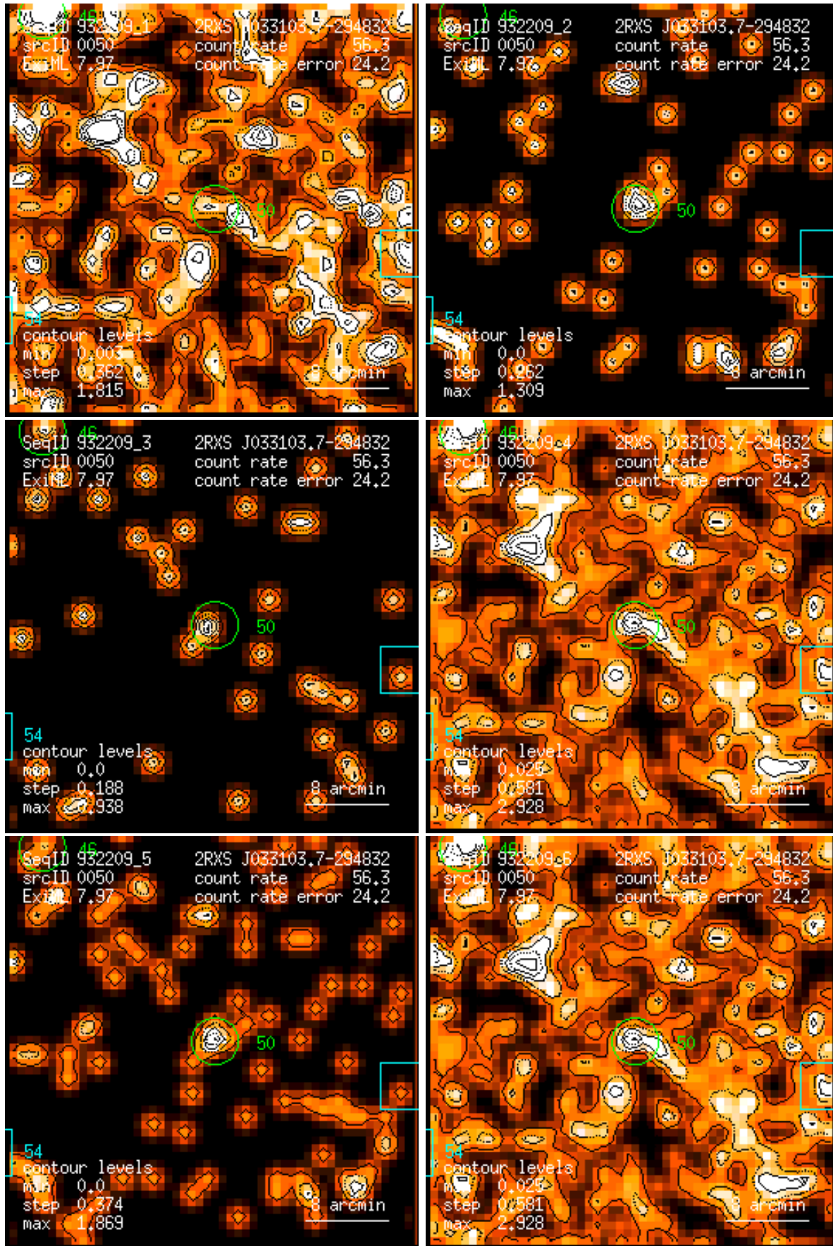
Figure 50: RASS 932209: detection 0050: band rate images, Gaussian filter: (1) PSPC channels 11 – 41, (2) 52 – 90, (3) 91 – 201, (4) 11 – 235, (5) 52 – 201, (6) 11 – 201. Broad band rates in counts/ks. Band rate contour levels in counts/ks/arcmin 2 .
