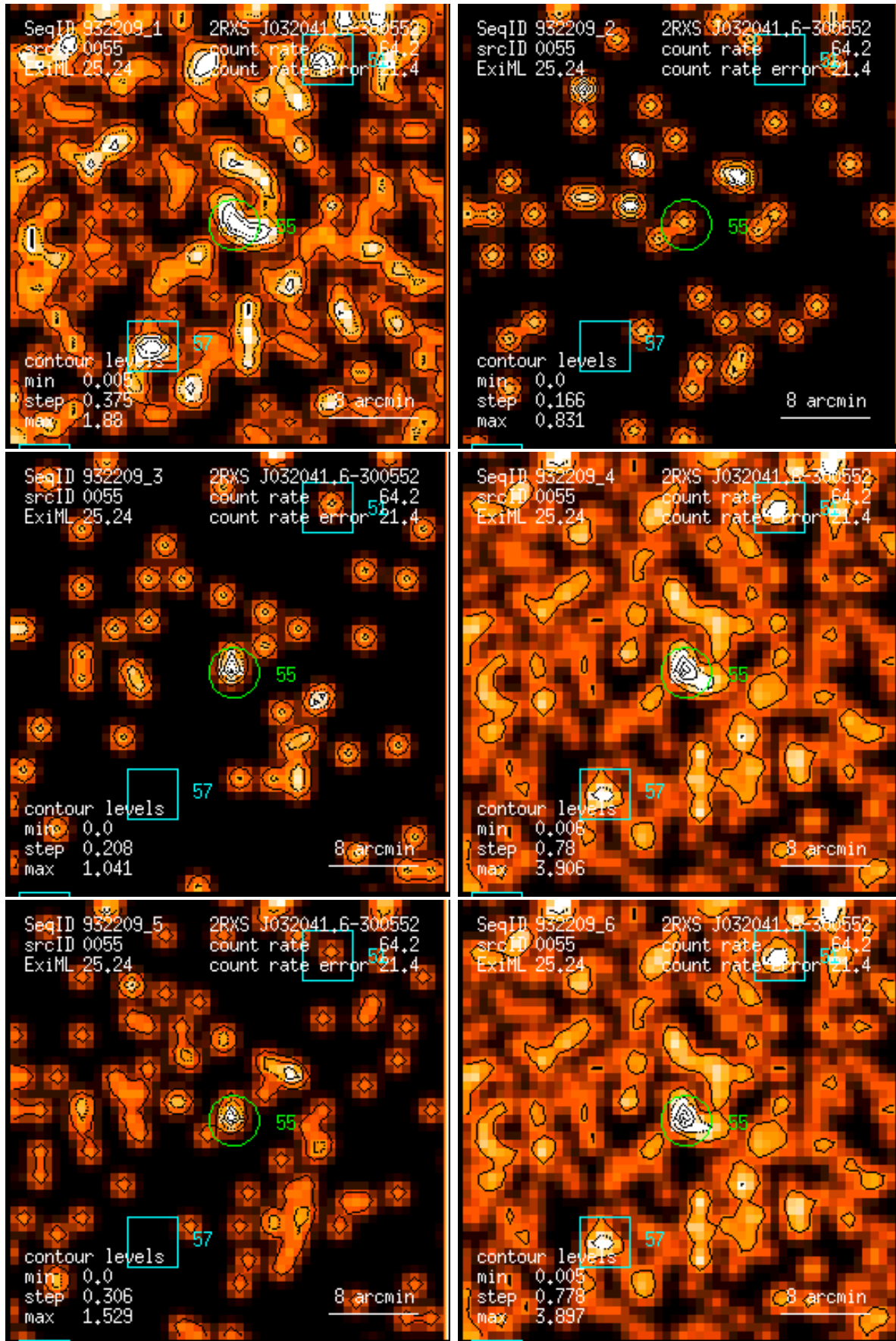
Figure 55: RASS 932209: detection 0055: band rate images, Gaussian filter: (1) PSPC channels 11 – 41, (2) 52 – 90, (3) 91 – 201, (4) 11 – 235, (5) 52 – 201, (6) 11 – 201. Broad band rates in counts/ks. Band rate contour levels in counts/ks/arcmin 2 .
