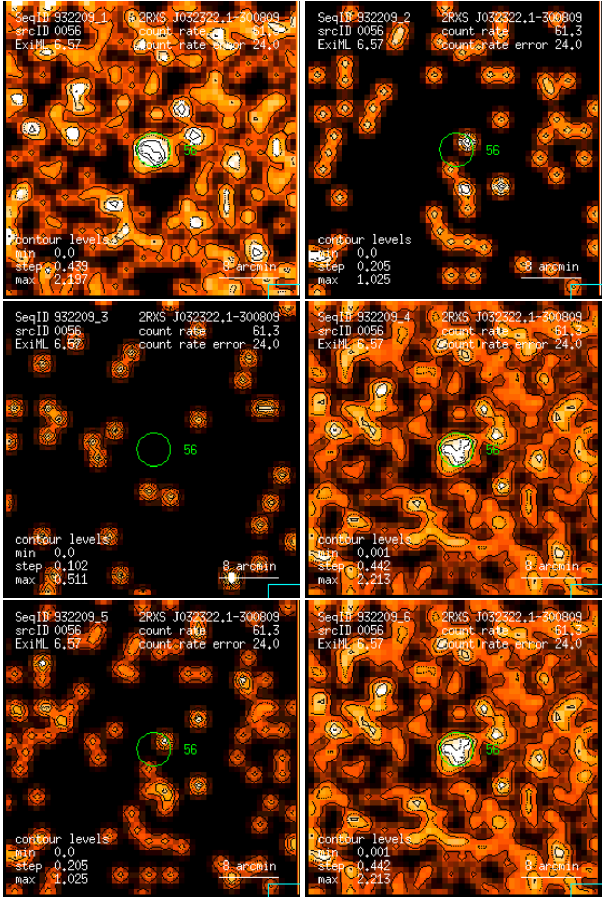
Figure 56: RASS 932209: detection 0056: band rate images, Gaussian filter: (1) PSPC channels 11 – 41, (2) 52 – 90, (3) 91 – 201, (4) 11 – 235, (5) 52 – 201, (6) 11 – 201. Broad band rates in counts/ks. Band rate contour levels in counts/ks/arcmin 2 .
