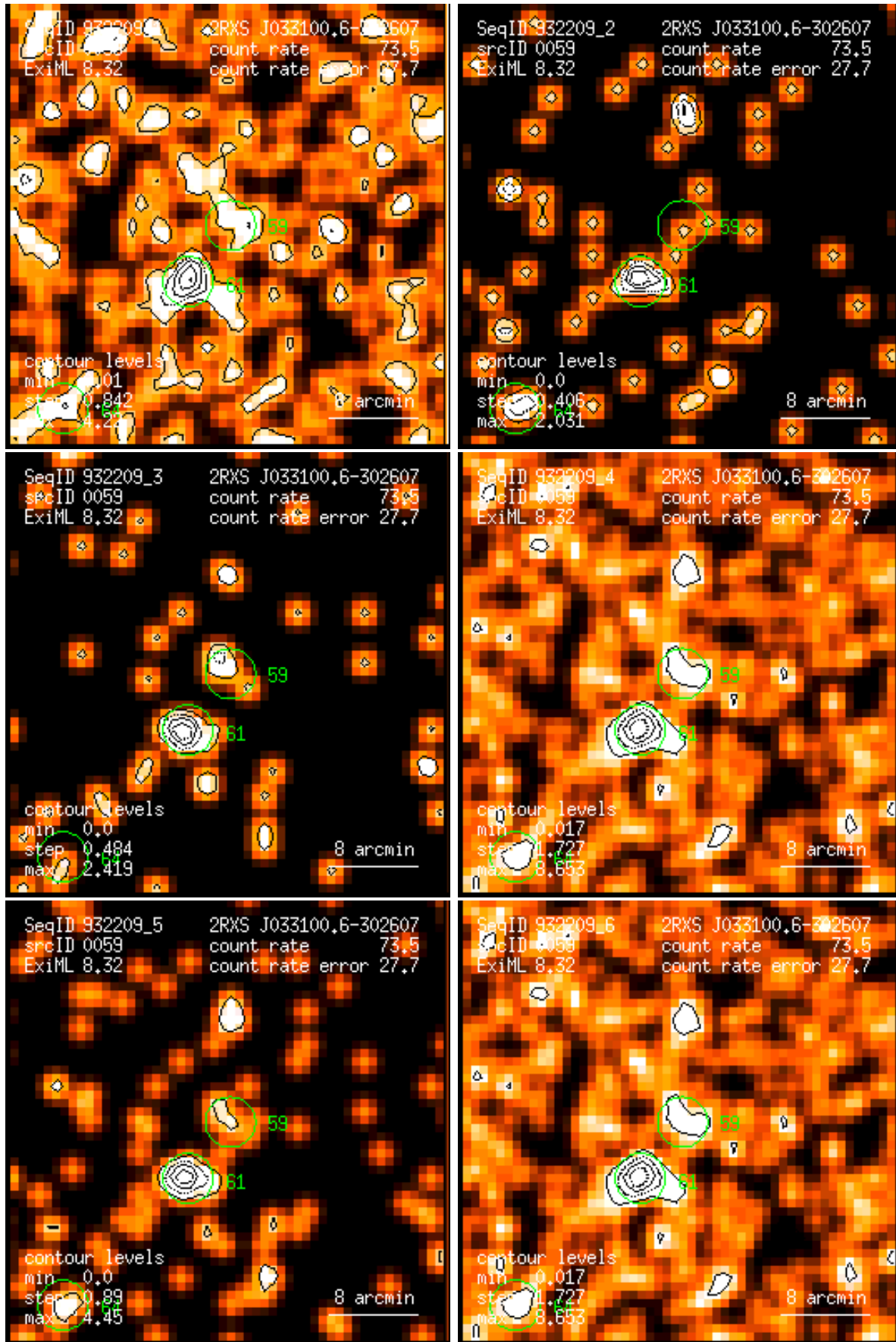
Figure 59: RASS 932209: detection 0059: band rate images, Gaussian filter: (1) PSPC channels 11 – 41, (2) 52 – 90, (3) 91 – 201, (4) 11 – 235, (5) 52 – 201, (6) 11 – 201. Broad band rates in counts/ks. Band rate contour levels in counts/ks/arcmin 2 .
