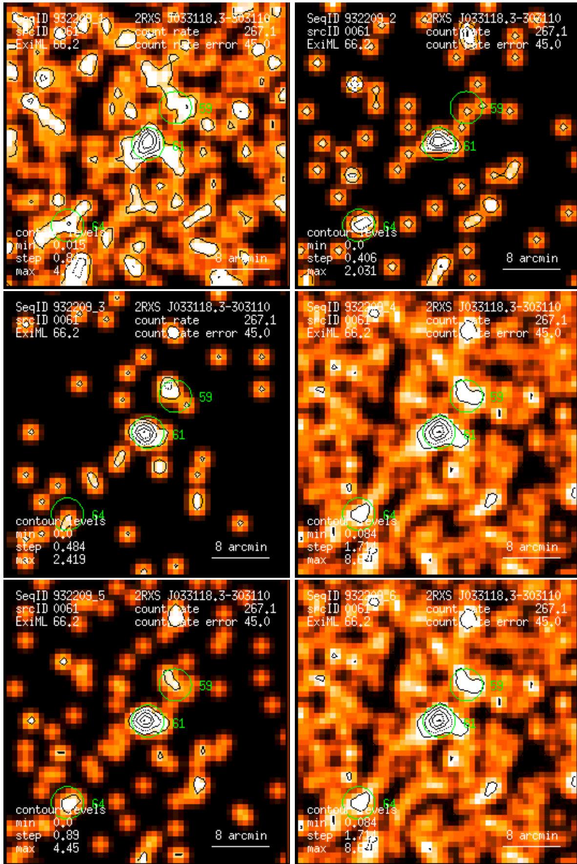
Figure 61: RASS 932209: detection 0061: band rate images, Gaussian filter: (1) PSPC channels 11 – 41, (2) 52 – 90, (3) 91 – 201, (4) 11 – 235, (5) 52 – 201, (6) 11 – 201. Broad band rates in counts/ks. Band rate contour levels in counts/ks/arcmin 2 .
