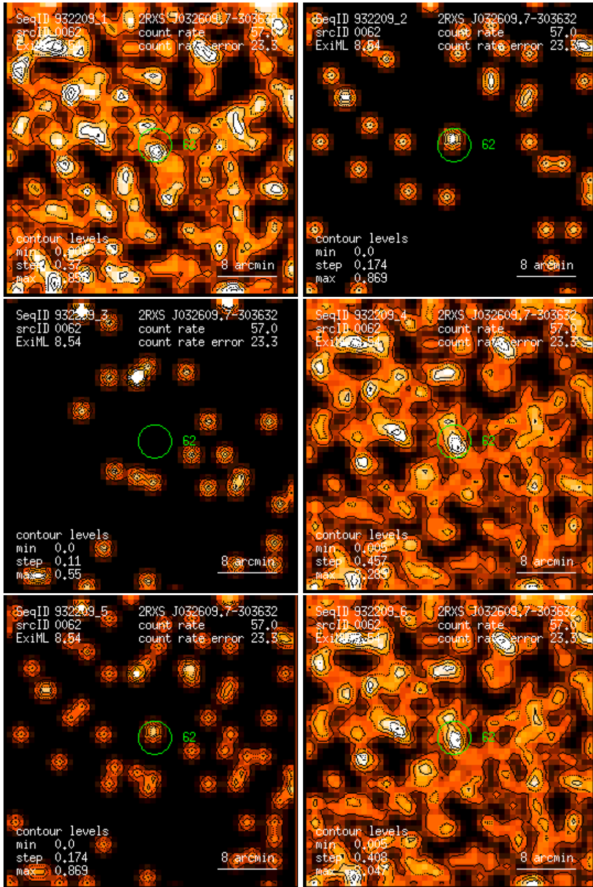
Figure 62: RASS 932209: detection 0062: band rate images, Gaussian filter: (1) PSPC channels 11 – 41, (2) 52 – 90, (3) 91 – 201, (4) 11 – 235, (5) 52 – 201, (6) 11 – 201. Broad band rates in counts/ks. Band rate contour levels in counts/ks/arcmin 2 .
