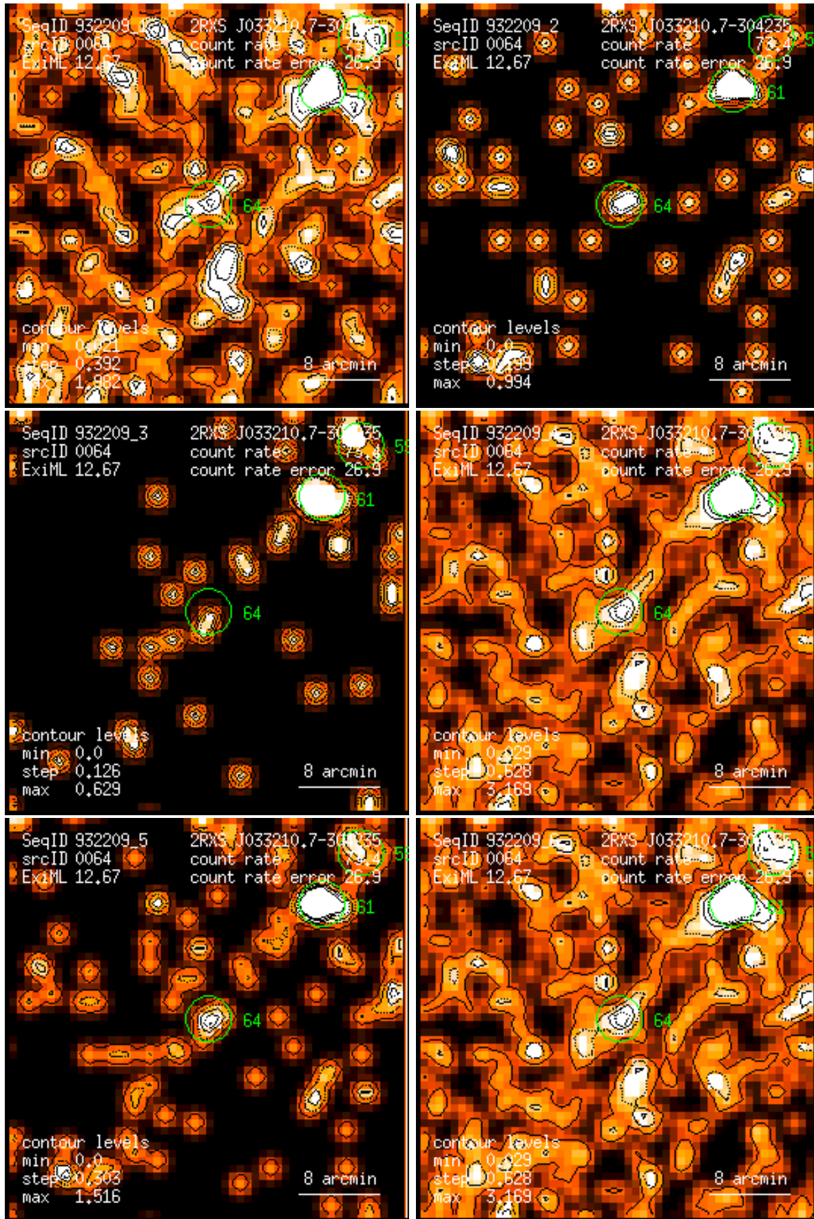
Figure 64: RASS 932209: detection 0064: band rate images, Gaussian filter: (1) PSPC channels 11 – 41, (2) 52 – 90, (3) 91 – 201, (4) 11 – 235, (5) 52 – 201, (6) 11 – 201. Broad band rates in counts/ks. Band rate contour levels in counts/ks/arcmin 2 .
