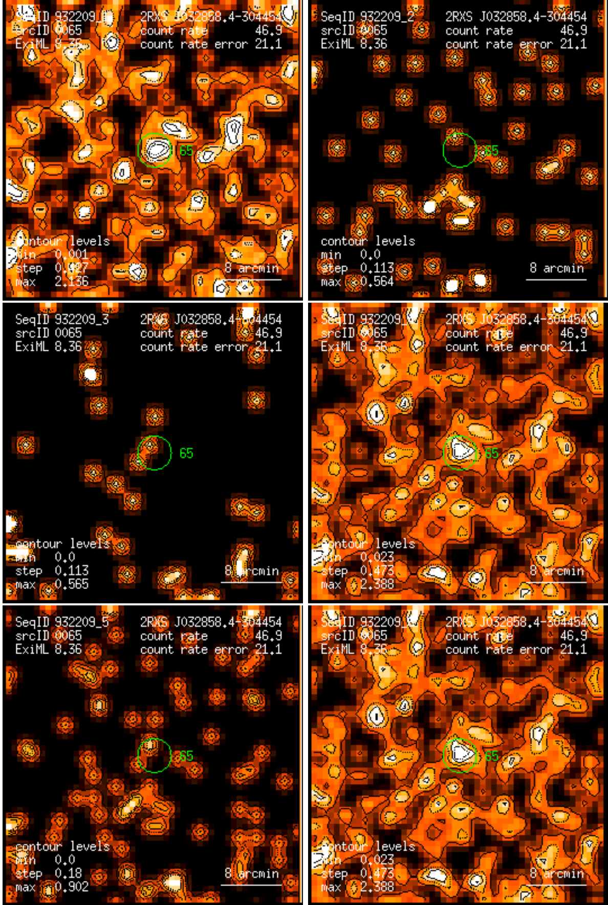
Figure 65: RASS 932209: detection 0065: band rate images, Gaussian filter: (1) PSPC channels 11 – 41, (2) 52 – 90, (3) 91 – 201, (4) 11 – 235, (5) 52 – 201, (6) 11 – 201. Broad band rates in counts/ks. Band rate contour levels in counts/ks/arcmin 2 .
