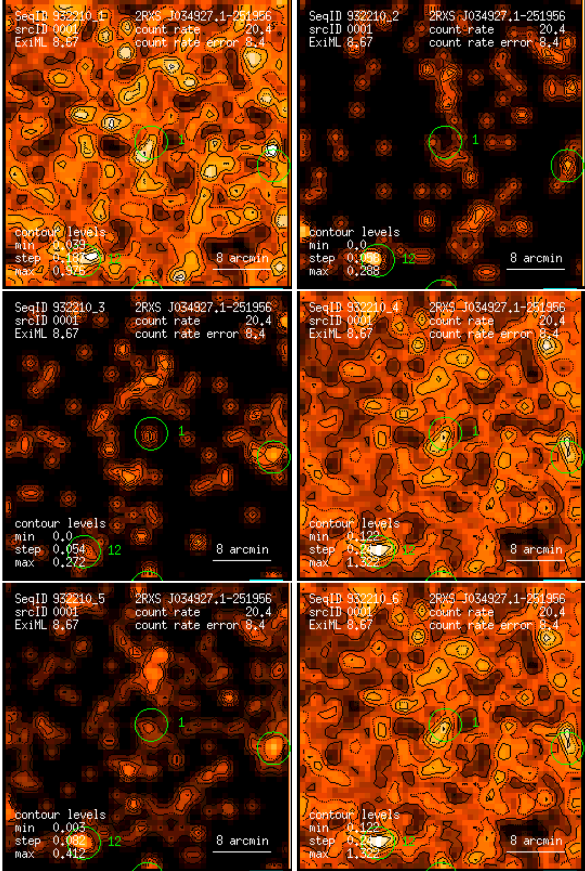
Figure 1: RASS 932210: detection 0001: band rate images, Gaussian filter: (1) PSPC channels 11 – 41, (2) 52 – 90, (3) 91 – 201, (4) 11 – 235, (5) 52 – 201, (6) 11 – 201. Broad band rates in counts/ks. Band rate contour levels in counts/ks/arcmin 2 .
