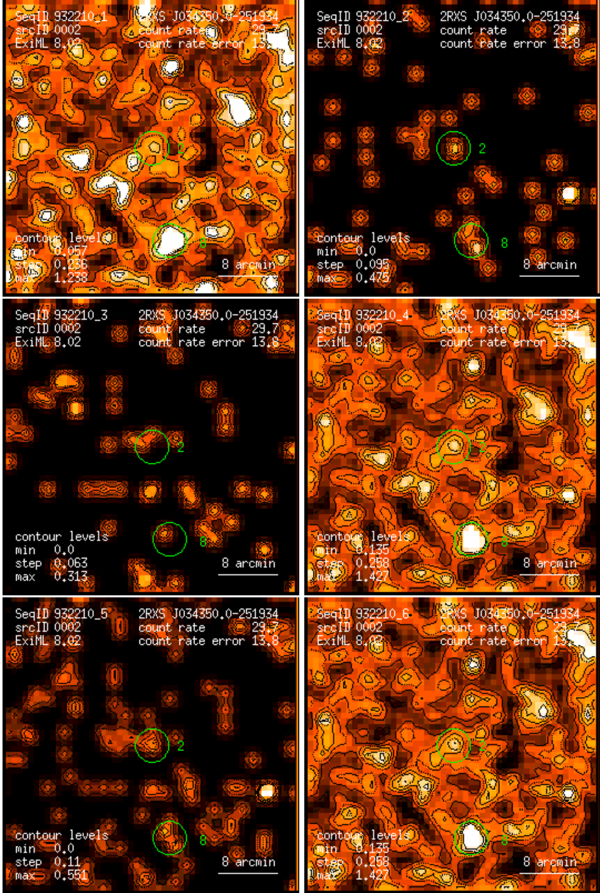
Figure 2: RASS 932210: detection 0002: band rate images, Gaussian filter: (1) PSPC channels 11 – 41, (2) 52 – 90, (3) 91 – 201, (4) 11 – 235, (5) 52 – 201, (6) 11 – 201. Broad band rates in counts/ks. Band rate contour levels in counts/ks/arcmin 2 .
