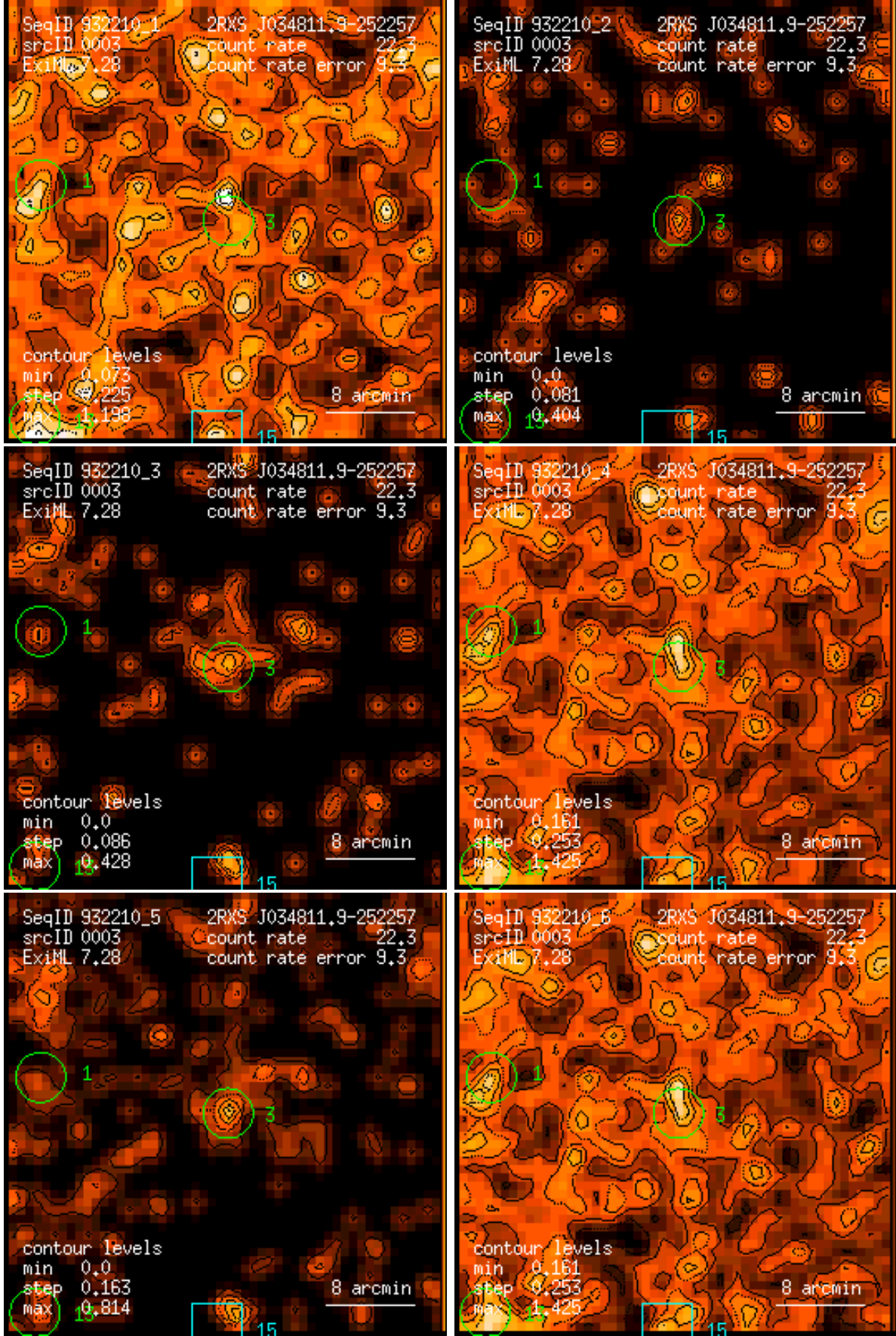
Figure 3: RASS 932210: detection 0003: band rate images, Gaussian filter: (1) PSPC channels 11 – 41, (2) 52 – 90, (3) 91 – 201, (4) 11 – 235, (5) 52 – 201, (6) 11 – 201. Broad band rates in counts/ks. Band rate contour levels in counts/ks/arcmin 2 .
