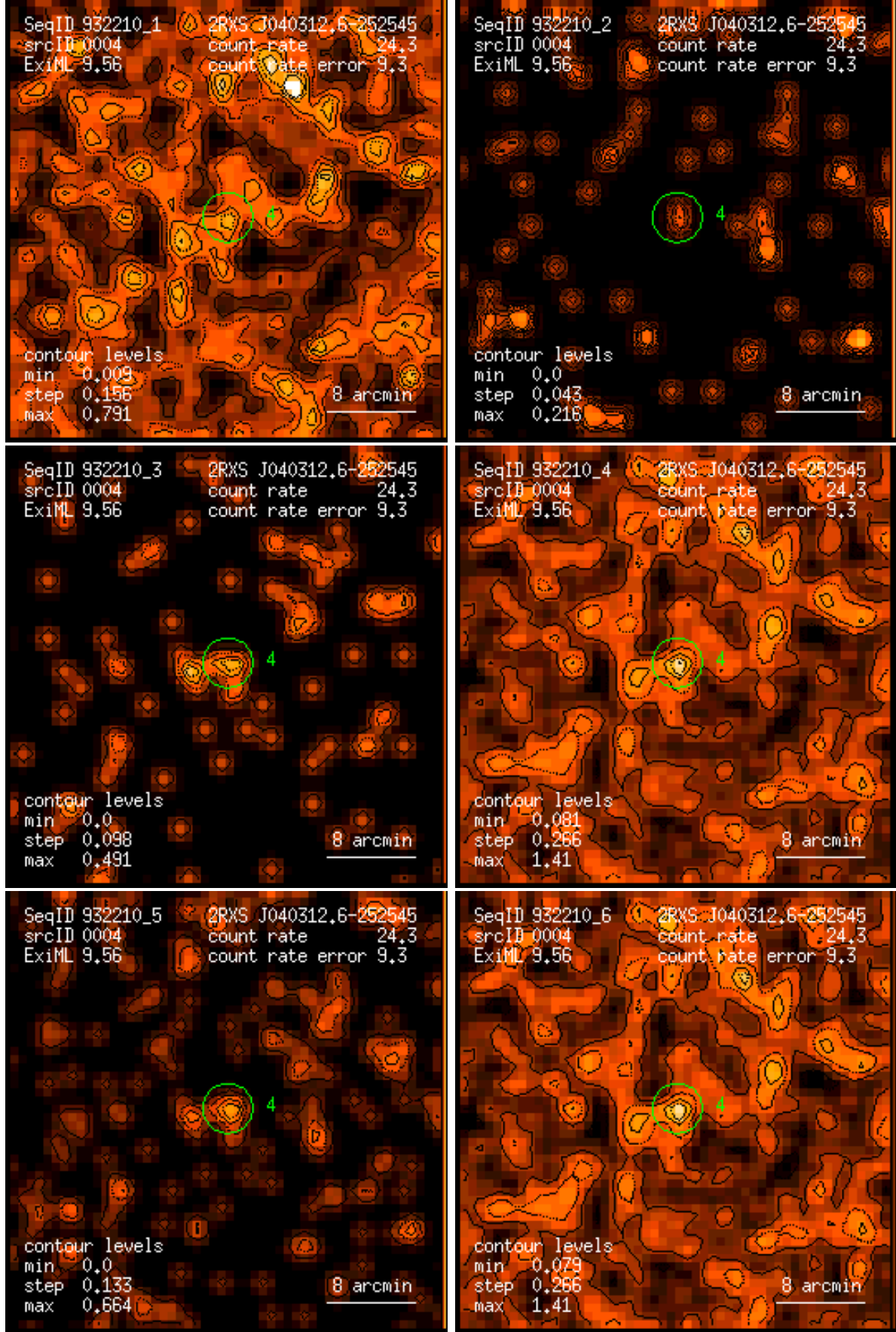
Figure 4: RASS 932210: detection 0004: band rate images, Gaussian filter: (1) PSPC channels 11 – 41, (2) 52 – 90, (3) 91 – 201, (4) 11 – 235, (5) 52 – 201, (6) 11 – 201. Broad band rates in counts/ks. Band rate contour levels in counts/ks/arcmin 2 .
