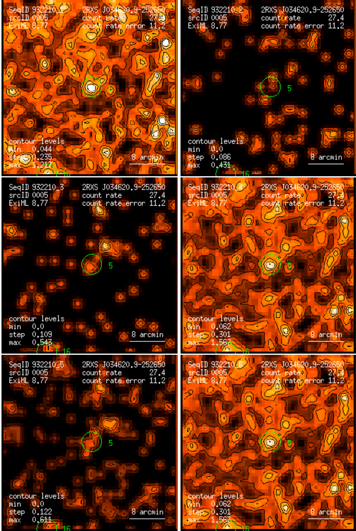
Figure 5: RASS 932210: detection 0005: band rate images, Gaussian filter: (1) PSPC channels 11 – 41, (2) 52 – 90, (3) 91 – 201, (4) 11 – 235, (5) 52 – 201, (6) 11 – 201. Broad band rates in counts/ks. Band rate contour levels in counts/ks/arcmin 2 .
