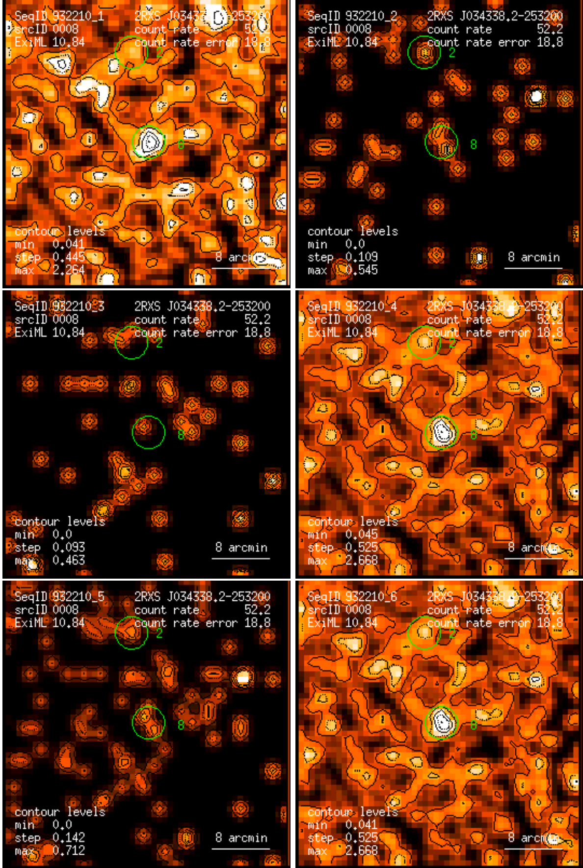
Figure 8: RASS 932210: detection 0008: band rate images, Gaussian filter: (1) PSPC channels 11 – 41, (2) 52 – 90, (3) 91 – 201, (4) 11 – 235, (5) 52 – 201, (6) 11 – 201. Broad band rates in counts/ks. Band rate contour levels in counts/ks/arcmin 2 .
