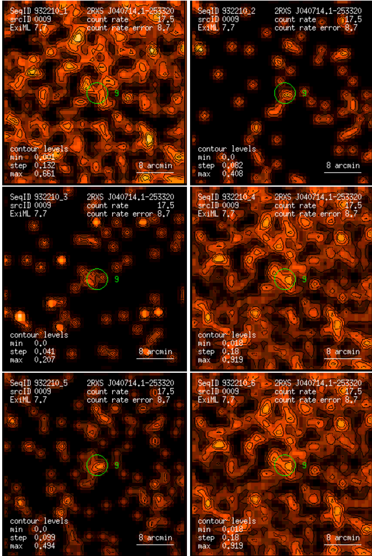
Figure 9: RASS 932210: detection 0009: band rate images, Gaussian filter: (1) PSPC channels 11 – 41, (2) 52 – 90, (3) 91 – 201, (4) 11 – 235, (5) 52 – 201, (6) 11 – 201. Broad band rates in counts/ks. Band rate contour levels in counts/ks/arcmin 2 .
