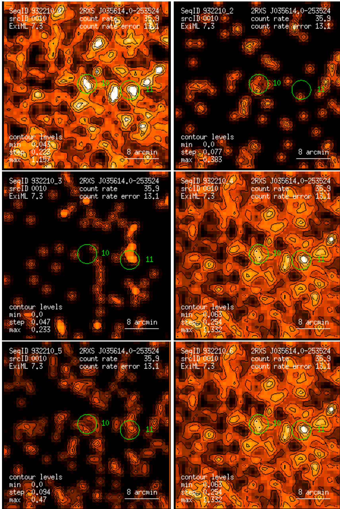
Figure 10: RASS 932210: detection 0010: band rate images, Gaussian filter: (1) PSPC channels 11 – 41, (2) 52 – 90, (3) 91 – 201, (4) 11 – 235, (5) 52 – 201, (6) 11 – 201. Broad band rates in counts/ks. Band rate contour levels in counts/ks/arcmin 2 .
