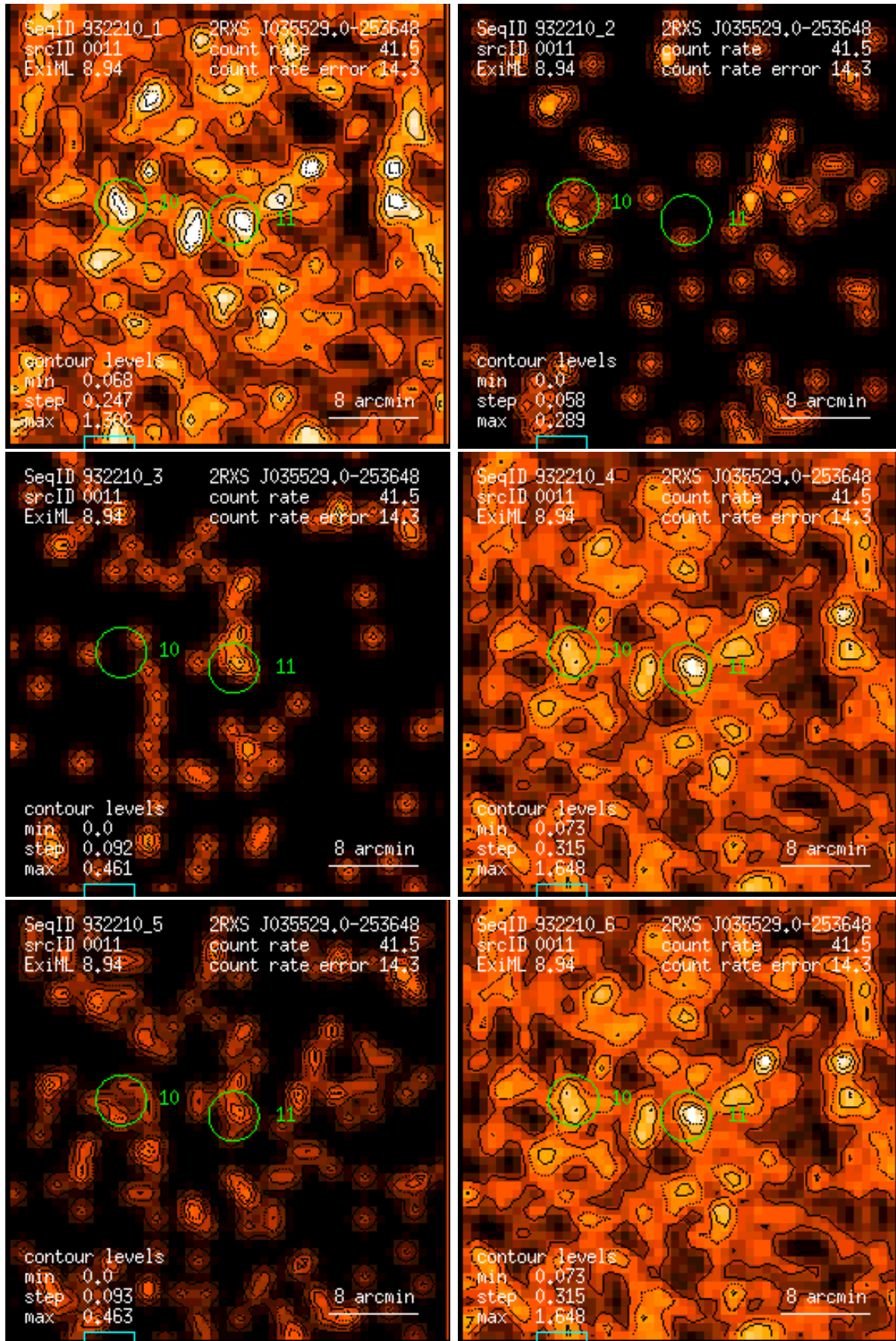
Figure 11: RASS 932210: detection 0011: band rate images, Gaussian filter: (1) PSPC channels 11 – 41, (2) 52 – 90, (3) 91 – 201, (4) 11 – 235, (5) 52 – 201, (6) 11 – 201. Broad band rates in counts/ks. Band rate contour levels in counts/ks/arcmin 2 .
