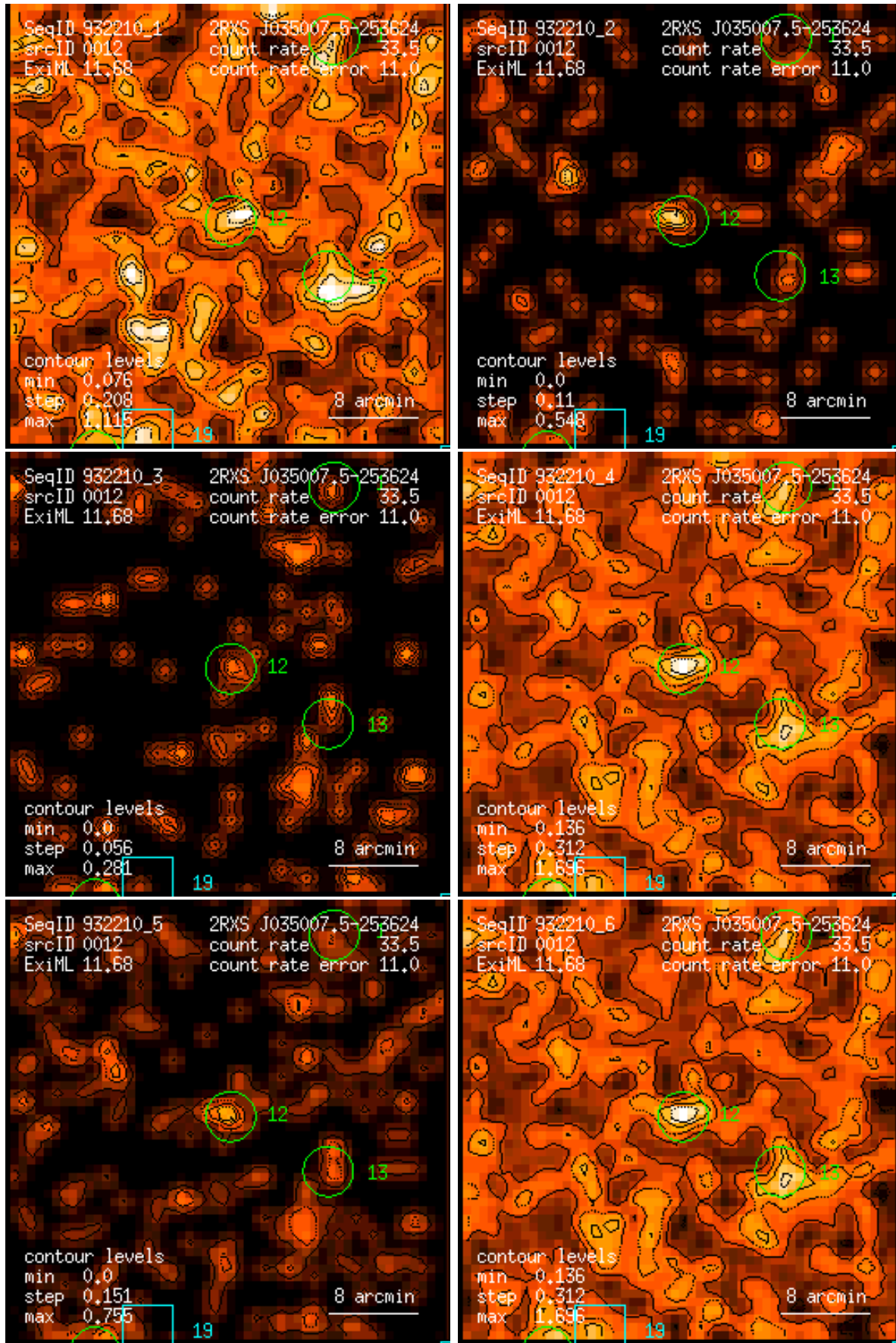
Figure 12: RASS 932210: detection 0012: band rate images, Gaussian filter: (1) PSPC channels 11 – 41, (2) 52 – 90, (3) 91 – 201, (4) 11 – 235, (5) 52 – 201, (6) 11 – 201. Broad band rates in counts/ks. Band rate contour levels in counts/ks/arcmin 2 .
