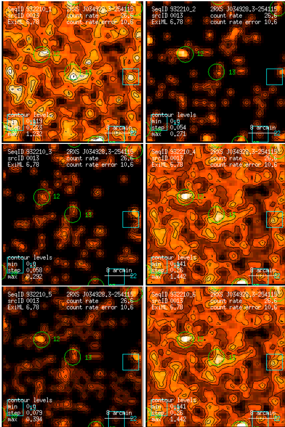
Figure 13: RASS 932210: detection 0013: band rate images, Gaussian filter: (1) PSPC channels 11 – 41, (2) 52 – 90, (3) 91 – 201, (4) 11 – 235, (5) 52 – 201, (6) 11 – 201. Broad band rates in counts/ks. Band rate contour levels in counts/ks/arcmin 2 .
